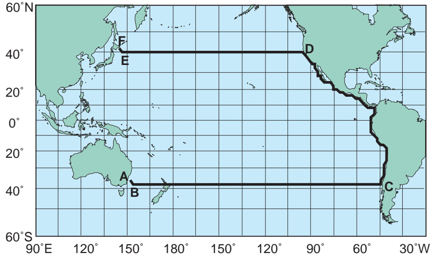
Figure 1. The horseshoe integration path ABCDEF in the throughflow model study (paper #4). Sections AB and EF are perpendicular to the boundary currents, whereas BC and ED are zonal sections. The integration of the COAD wind stress was done in 2š squares.
