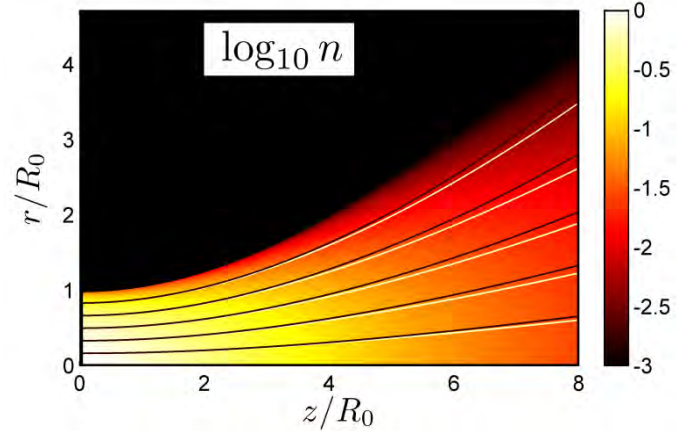
Fig.1. Logarithmic map of the normalized plasma density and pairs of electron (dark) and ion (light) streamtubes.
