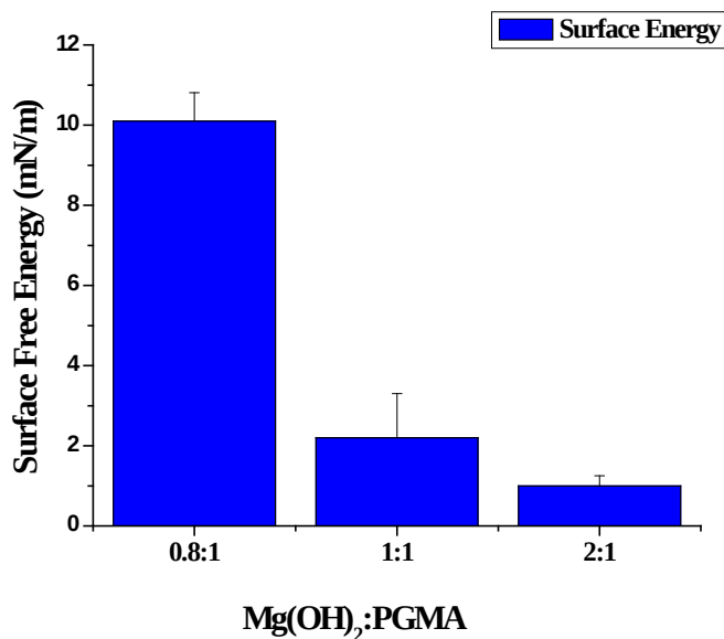
Figure 41. Surface Energy of Si Wafer Surfaces Coated with Different Mg(OH) 2 Suspensions in PGMA Solution and Mixed at Different Ratios
