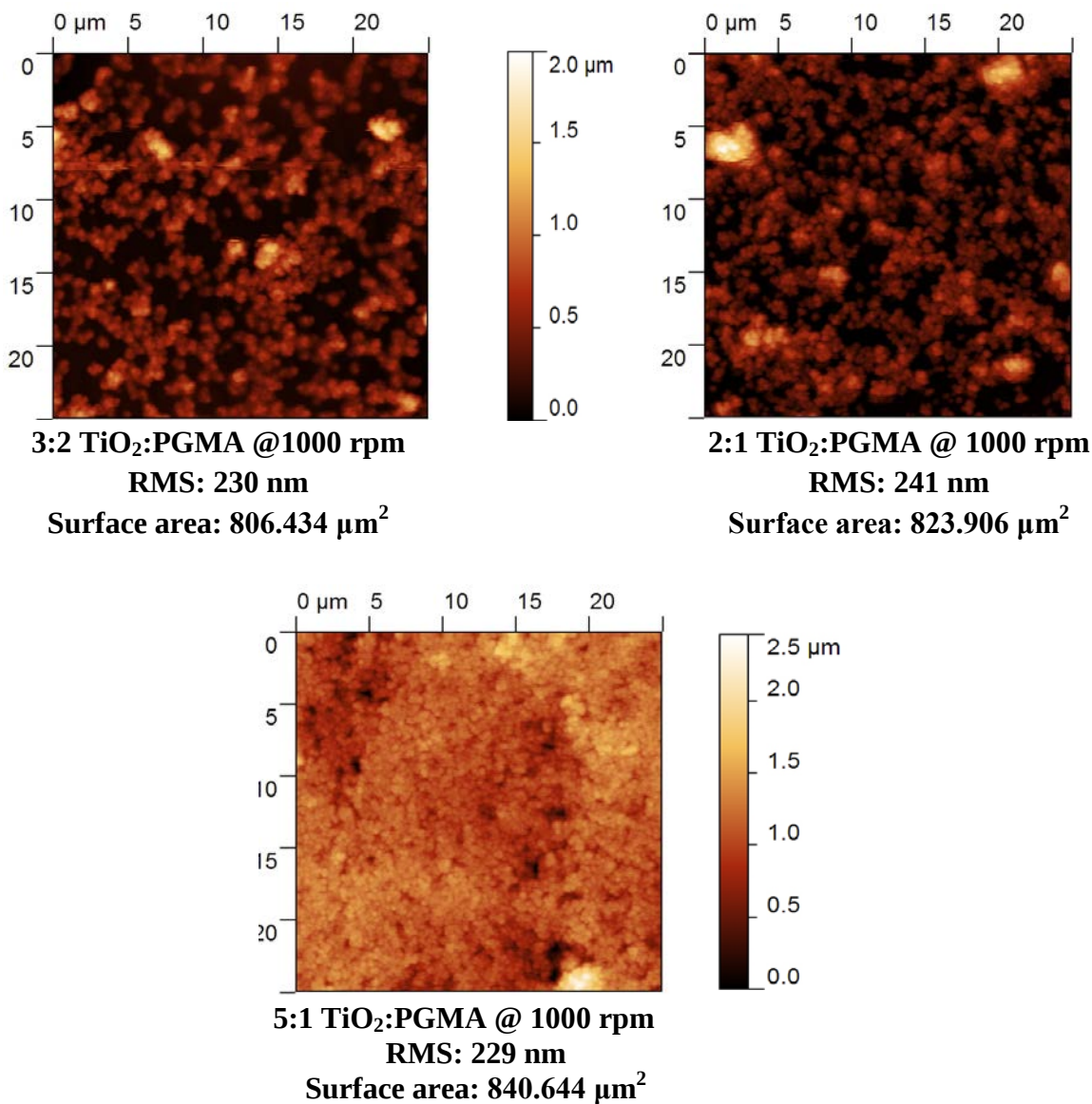
Figure 37. AFM Images of Si Wafers Spin Coated with TiO 2 Suspensions in PGMA Solution with Different Nanoparticle-to-PGMA Ratios RMS indicates roughness.
