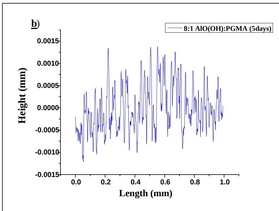
Figure 44. Profilometer Images of PFDOA-Treated AlO(OH)–PGMA Coatings after Shaking for 5 Days: a) RMS Roughness = 0.91 \mu\text{m} (1:1 AlO(OH):PGMA Suspension; b) RMS Roughness = 0.52 \mu\text{m} (8:1 AlO(OH):PGMA Suspension)
