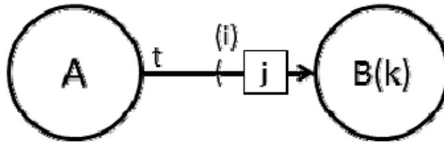
Figure 6. Event Graph with Parameter Passing (From Buss, 2001a)
