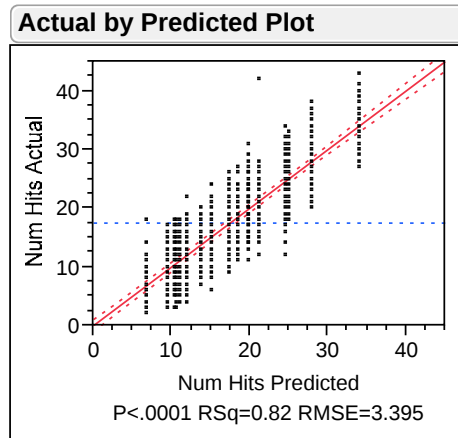
Figure 20. Actual by Predicted Plot for Full Factorial Regression Model for Number of Hits
