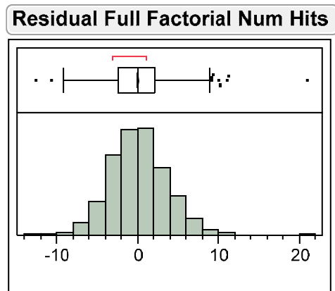
Figure 23. Residuals of Full Factorial Model for Number of Hits
