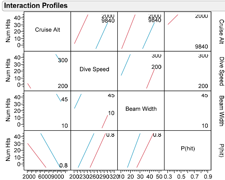
Figure 24. Interaction Profiler of Full Factorial Model for Number of Hits
