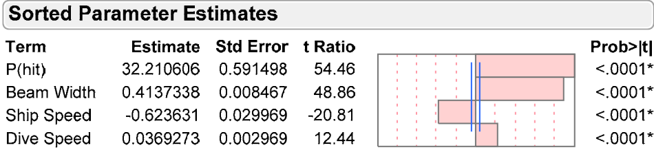
Figure 18. Sorted Parameter Estimates of Main Effects Model for Number of Hits
