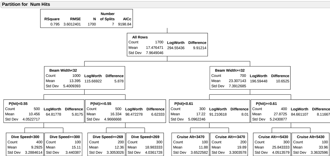
Figure 25. Partition Tree Model for Number of Hits
