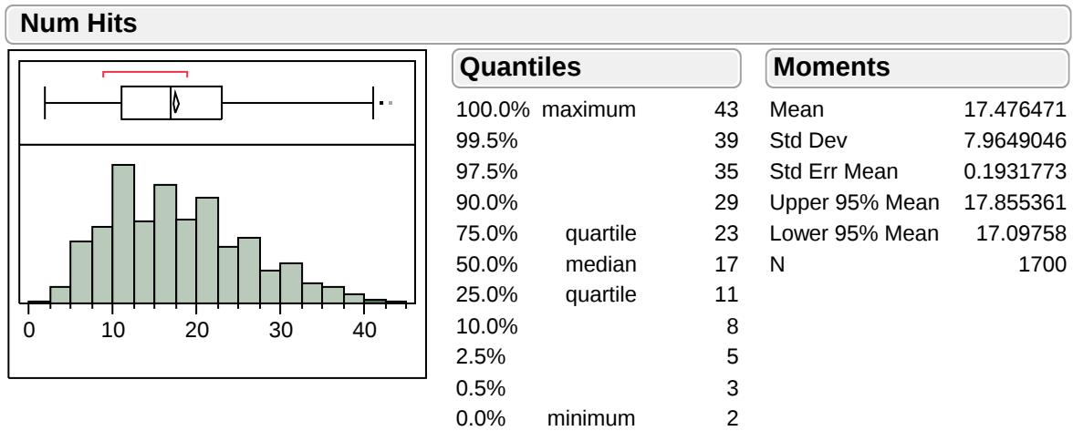
Figure 15. Distribution of Number of Hits
