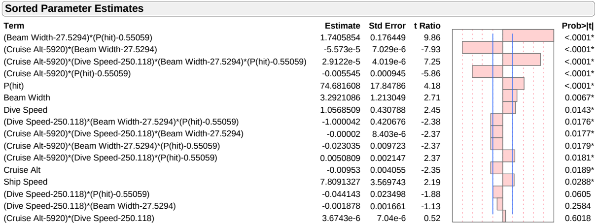
Figure 22. Sorted Parameter Estimates for Full Factorial Regression of Number of Hits
