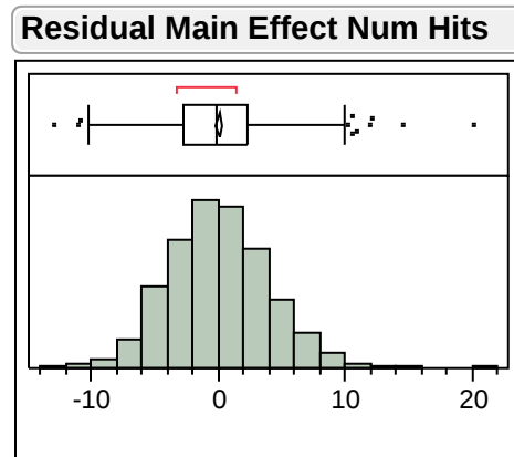
Figure 19. Residuals of Main Effects Model for Number of Hits
