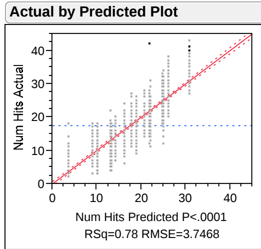
Figure 16. Actual by Predicted Plot of Main Effects Model for Number of Hits
