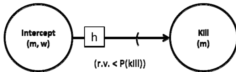
Figure 14. Potential Defensive Weapon Adjudicator Event Graph
