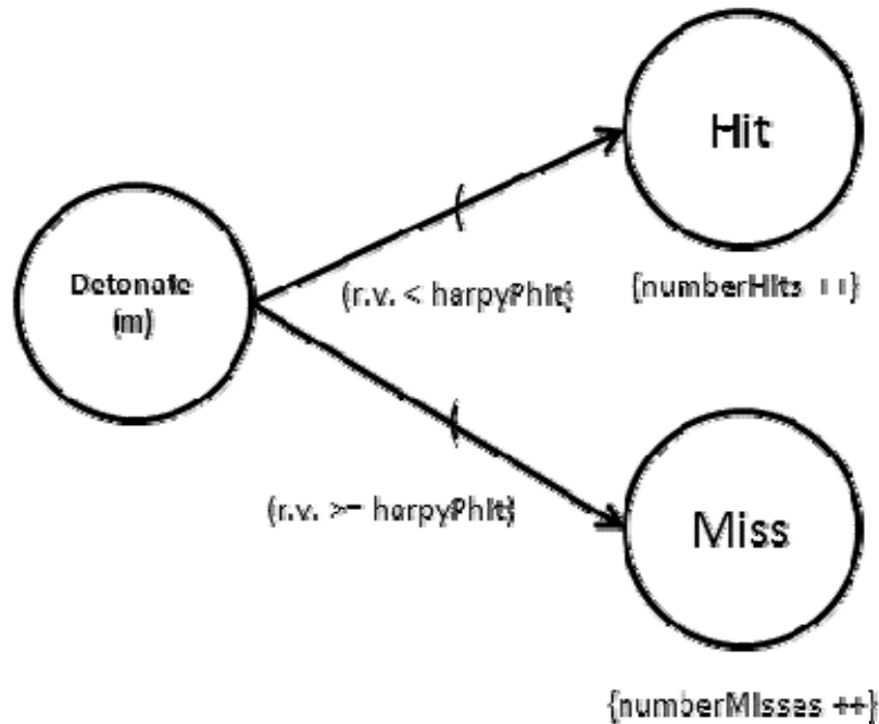
Figure 11. SimpleHarpyAdjudicator Event Graph
