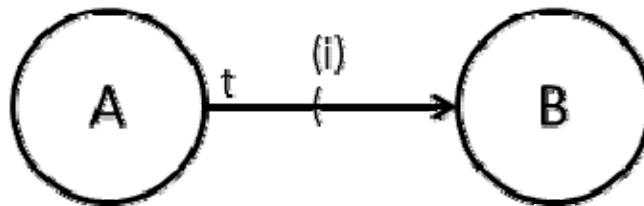
Figure 4. Basic Event Graph Construct (From Buss, 2001a)
