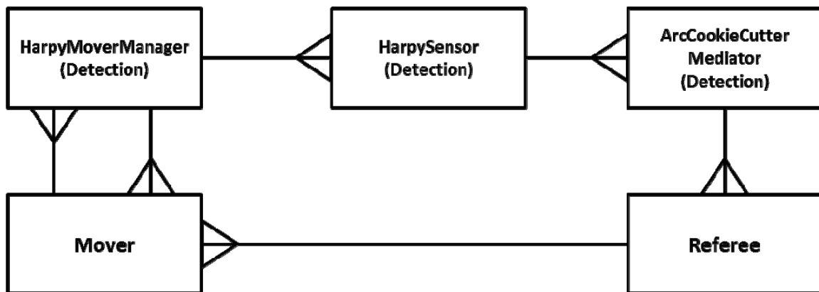
Figure 10. Listeners Associated with Harpy Detections
