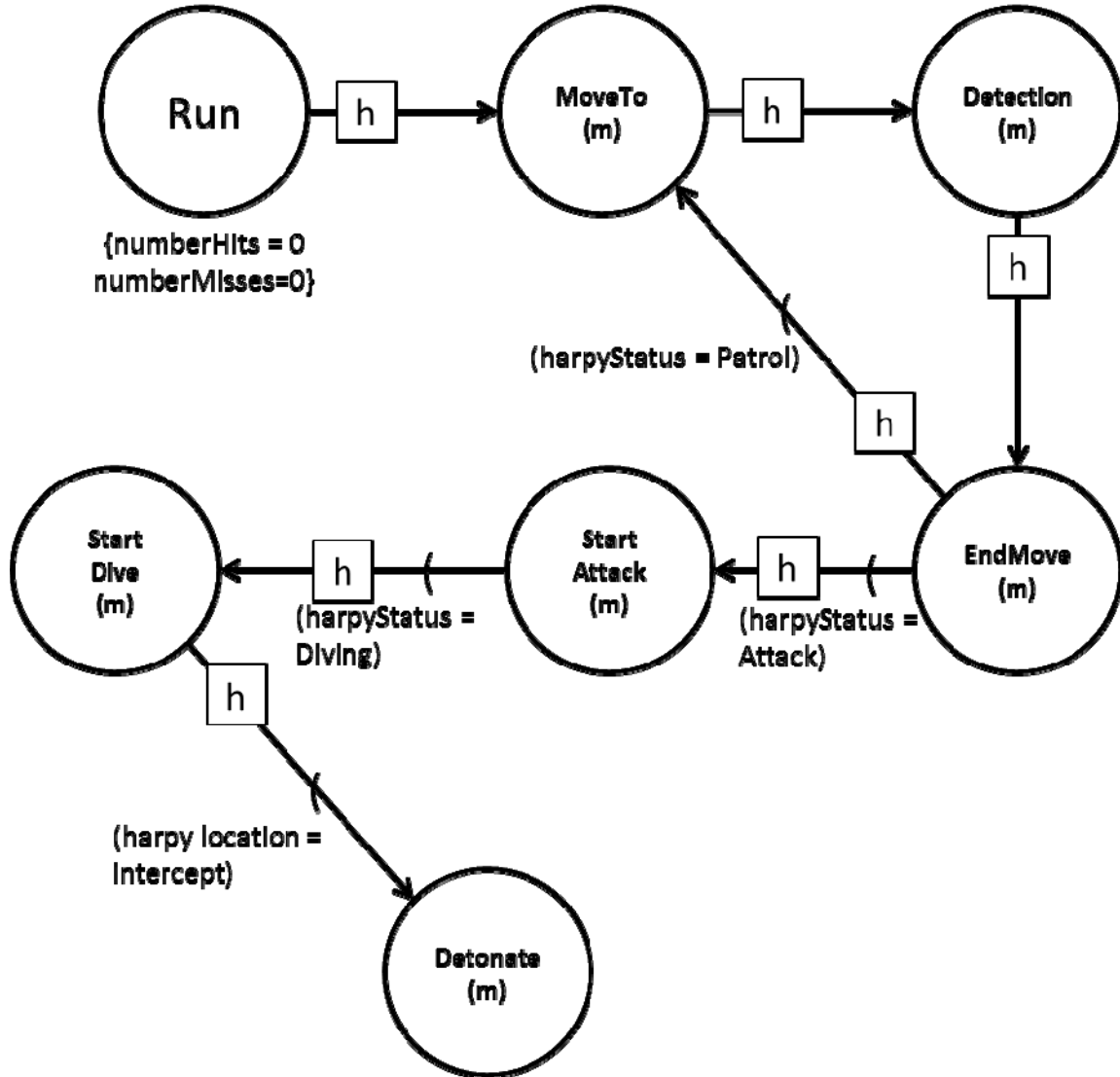
Figure 9. HarpyMoverManager Event Graph
