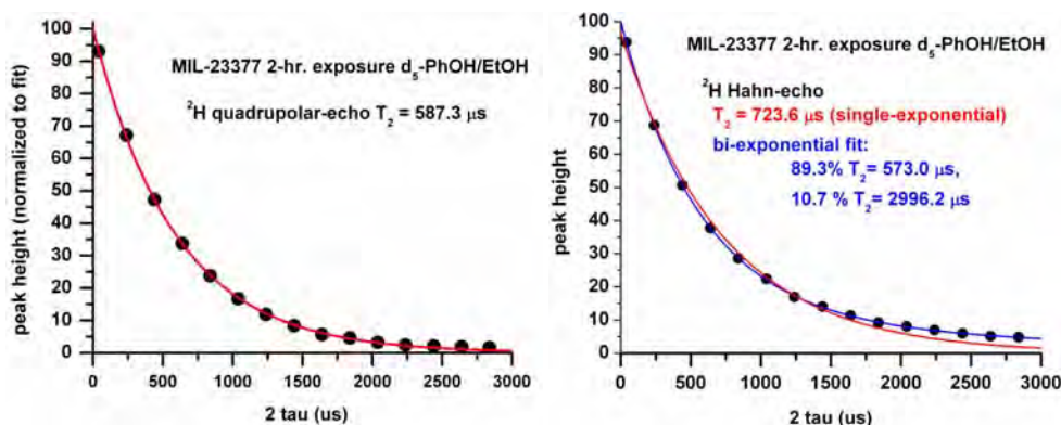
Figure 46: ^2\text{H} decay times at 24^\circ \text{C} of MIL-PRF-23377 epoxy primer exposed 2 hours to \text{d}_5 -PhOH/EtOH, as measured by two different echo pulse sequences (see text). The single-exponential fit on the right is systematically lower than the experimental data points, unlike the biexponential fit.
