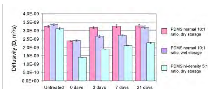
Figure 5. Experimentally determined oxygen diffusivity through 1 mm thick PDMS membranes as a function of surface properties and storage conditions. Note: 1) normal and high density PDMS have almost identical O 2 diffusivities in native state; 2) initial plasma treatment significantly decreases O 2 diffusivity, in some cases by more than 50%; 3) original diffusivity values are fully restored in 3 days for normal PDMS stored in air, while hi-density PDMS does not recover in 3 weeks under the same storage conditions; storage under water (normal operating conditions for a bioreactor) delays recovery by 3 weeks. Error bars represent the 95% confidence interval based on 3 independent measurements with 3 different membranes.
