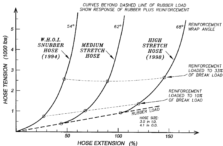
Figure 3. Hose stretch versus tension for several cord geometries.
