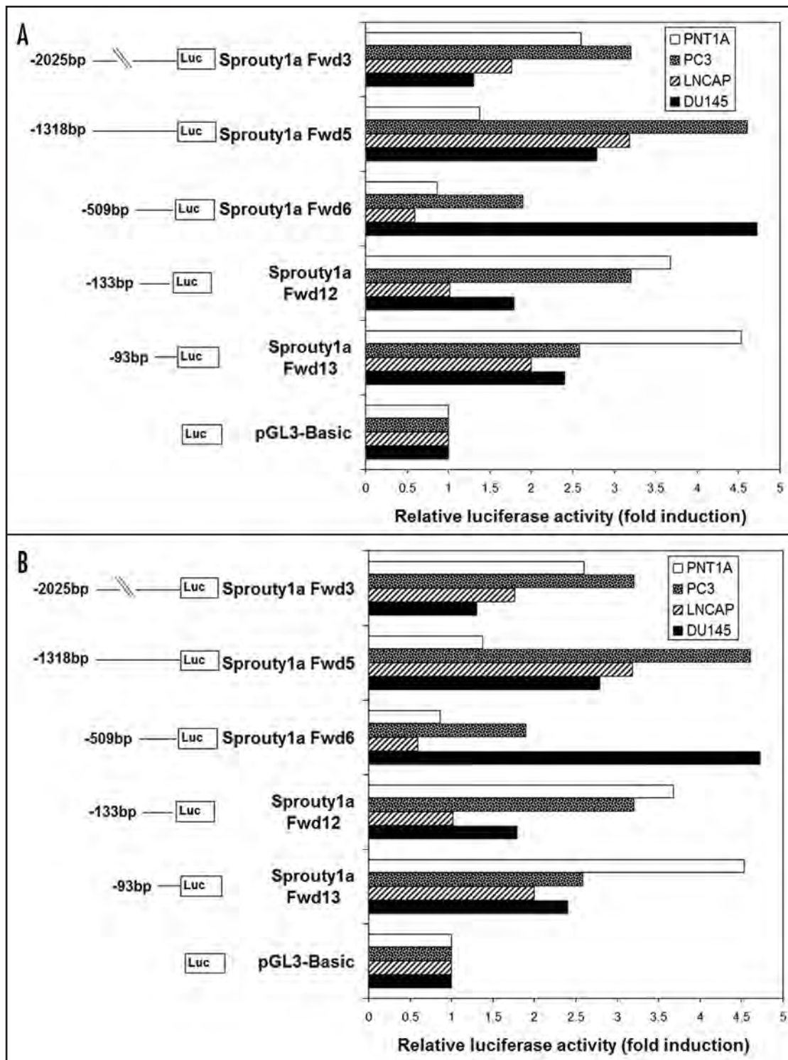
Figure 2. Progressive deletion analysis of the 5'-flanking region of splice variant 1a and 1b of the human Sprouty1 gene. The schematic diagrams represent a series of Sprouty1a (A) and Sprouty1b (B) gene constructs with variable 5'-ends as indicated. The luciferase activity was measured and normalized for transfection efficiency by dividing the measurement of the firefly luciferase activity by that of the \beta -galactosidase activity. The relative luciferase activities are represented as fold induction with respect to that obtained in cells transfected with the empty control vector (pGL3-Basic). Data represents the mean of triplicate experiments.
