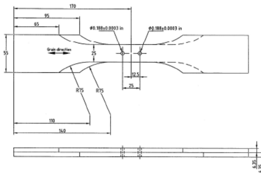
Figure A-7: P-3 Low-Load Transfer Joint Coupon
