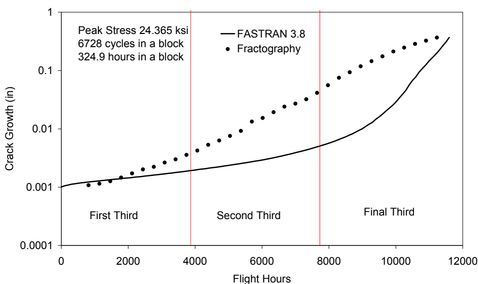
Figure 37: Experimental and FASTRAN predicted crack growth for F18 FT55m5 spectrum example
