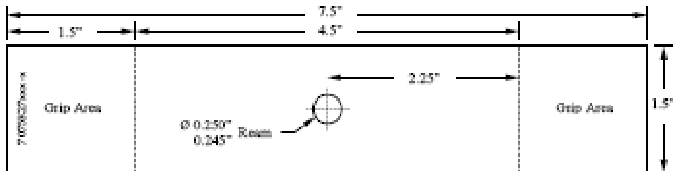
Figure A-6: P-3 Open Hole Coupon
