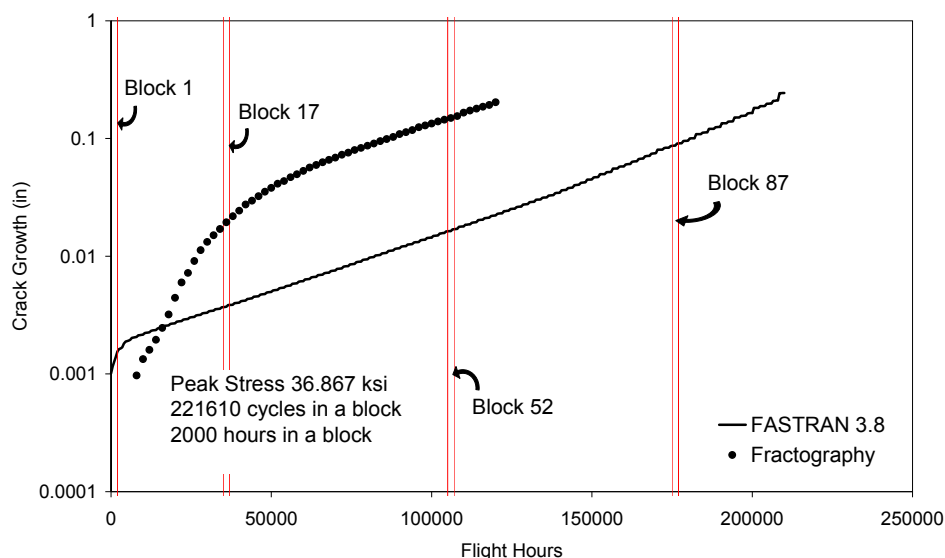
Figure 35: Experimental and FASTRAN predicted crack growth for F-111 D20 spectrum example
