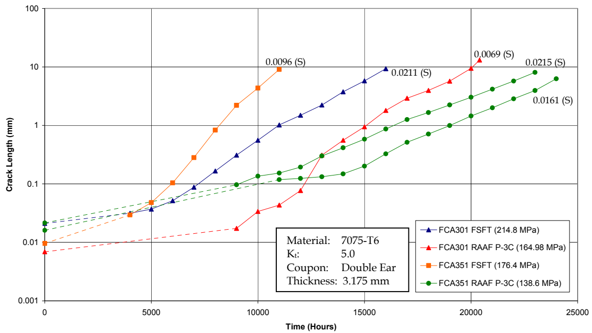
Figure 12: Crack Growth for different P-3C FCA301 and FCA351 Spectra – Double-Ear Coupons
