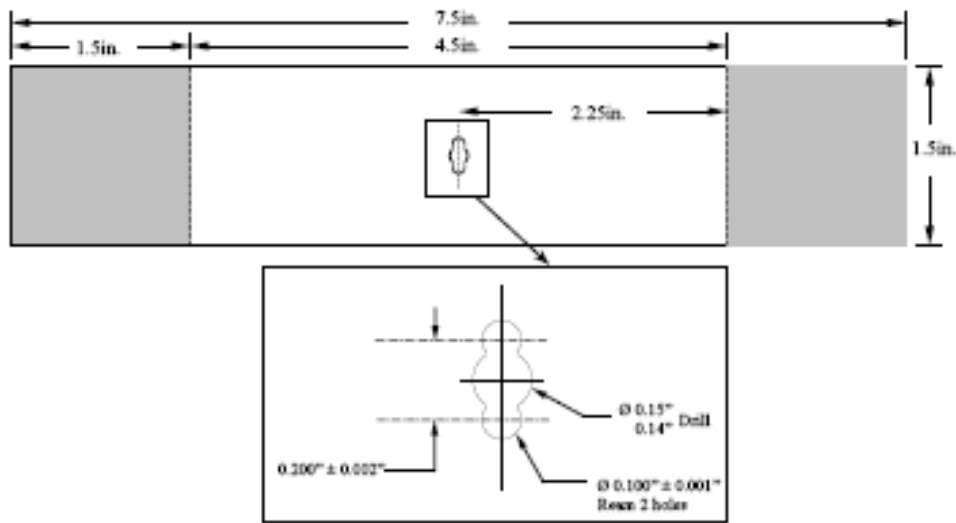
Figure A-5: P-3 High Kt Double-Ear Coupon
