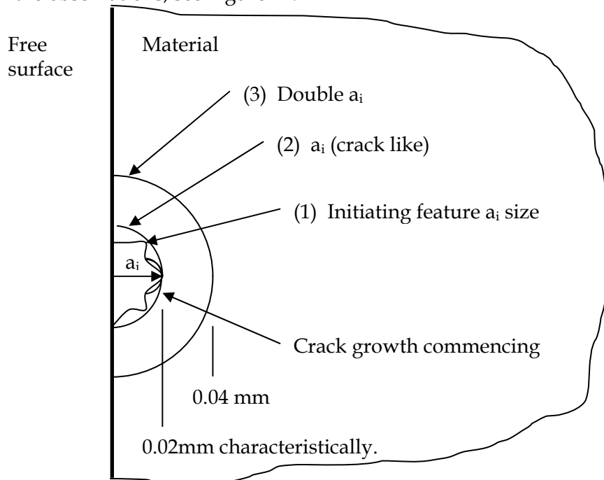
Figure 17: Crack commencement visualisation in stages (1), (2) and (3)
