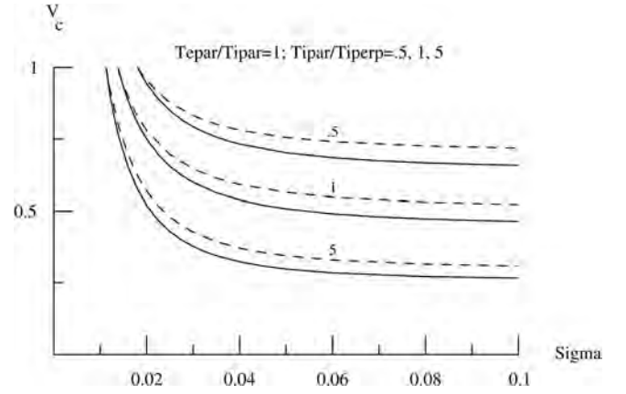
FIG. 10. Threshold (critical) value of electron drift speed, normalized to V_{e\parallel} and denoted by V_c , as a function of \omega_{pe}/\Omega_e = \sigma (Sigma) for T_{e\parallel}/T_{i\parallel} = 1 and selected values of T_{i\parallel}/T_{i\perp} . The solid curves represent results for bi-Maxwellian plasma and the dashed curves represent results for kappa-Maxwellian ( \kappa_e = \kappa_i = 3 ) plasma. The curves are labeled by the selected values of T_{i\parallel}/T_{i\perp} .
