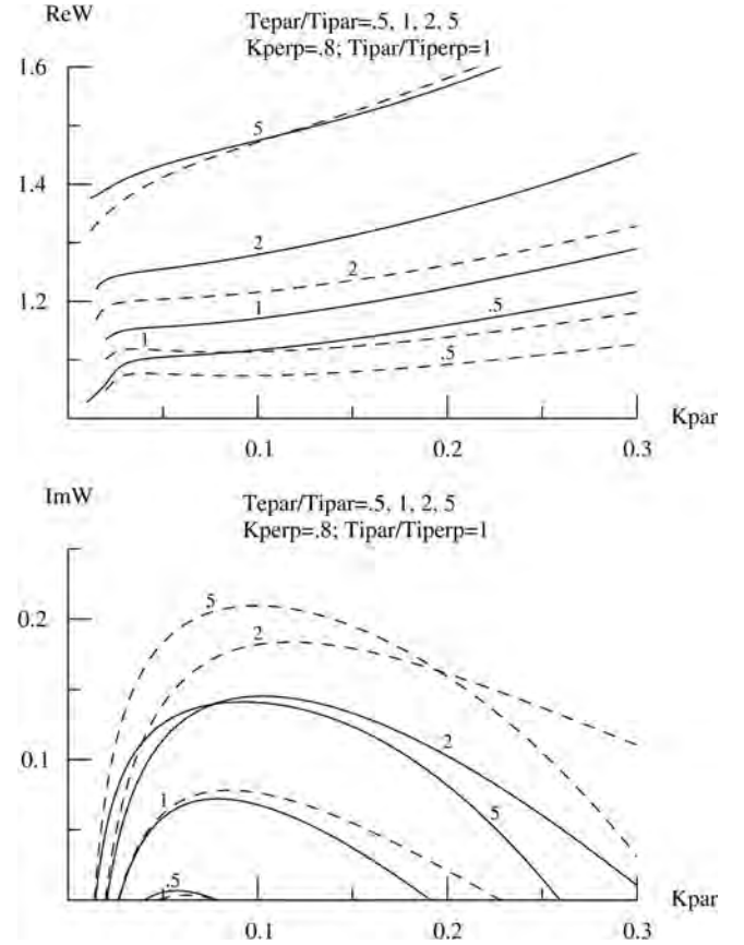
FIG. 8. (Top panel) \text{Re}W (\equiv \text{Re}\omega/\Omega_i) vs. K_\parallel (\equiv K_{\parallel\rho_i}) = k_\parallel \rho_i and (bottom panel) \text{Im}W (\equiv \text{Im}\omega/\Omega_i) vs. K_\parallel for \omega_{pe}/\Omega_e = 1/15 , V_0 (\equiv V_0/V_{e||}) = 1 , K_\perp (\equiv K_{\perp\rho_i}) = k_\perp \rho_i = 0.8 , T_{i||}/T_{i\perp} = 1 , and selected values of T_{e||}/T_{i||} . The solid curves represent results for bi-Maxwellian plasma and the dashed curves represent results for kappa-Maxwellian ( \kappa_e = \kappa_i = 3 ) plasma. The curves are labeled by the selected values of T_{e||}/T_{i||} .
