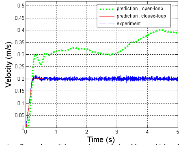
Fig. 4. Comparison of the open-loop and closed-loop vehicle velocities when the vehicle is commanded to 0.2 \text{ m/s} for straight-line movement on the lab vinyl surface
