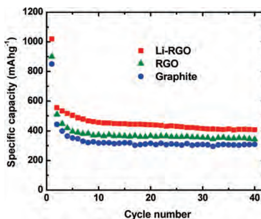
Figure 5. Variation in discharge capacity vs cycle number for graphite, RGO, and Li-RGO cycled at a current rate of 25 \text{ mA/g} between 3.0 and 0.02 \text{ V} vs \text{Li/Li}^+ in a 1 M solution of \text{LiPF}_6 in a 1:1 (v/v) mixture of ethylene carbonate (EC) and dimethyl carbonate (DMC) as the electrolyte.
