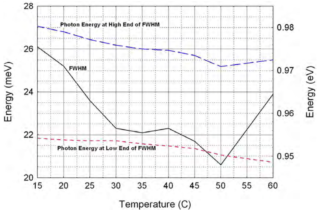
Figure 4.18: FWHM of the QD active region of a 50 \mu\text{m} diameter RCLED (SH118) in meV and the high and low end points at half maximum versus the device chuck temperature
