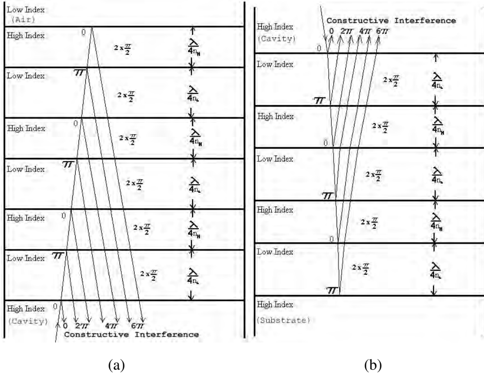
Figure 2.3: Constructive interference in a (a) top DBR mirror and a (b) bottom DBR mirror.
