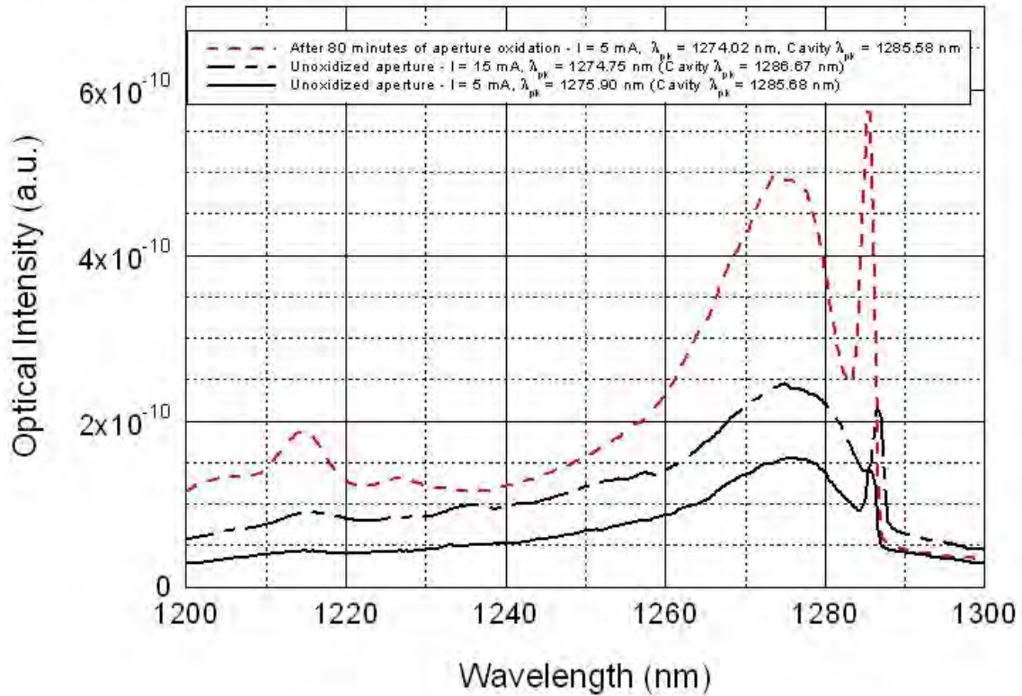
Figure 4.11: Output of a 25 μm V17 VCSEL prior to oxidation of the oxide aperture at drive currents of 5 mA and 15 mA, and after 80 minutes of oxidation at a current of 5 mA
