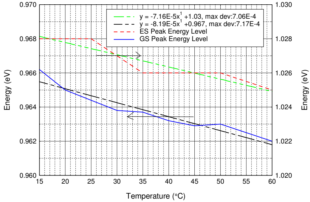
Figure 4.17: Peak energy levels of the ground state (GS) and excited state (ES) of the QD active region of a 50 \mu\text{m} RCLED (SH118) versus chuck temperature
