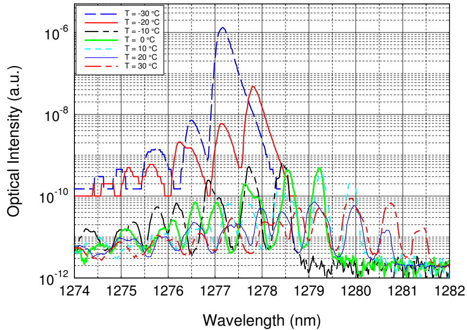
Figure 4.35: Output of a 15 \mu\text{m} DO177 VCSEL at I_d = 4 mA over various chuck temperatures in a log scale
