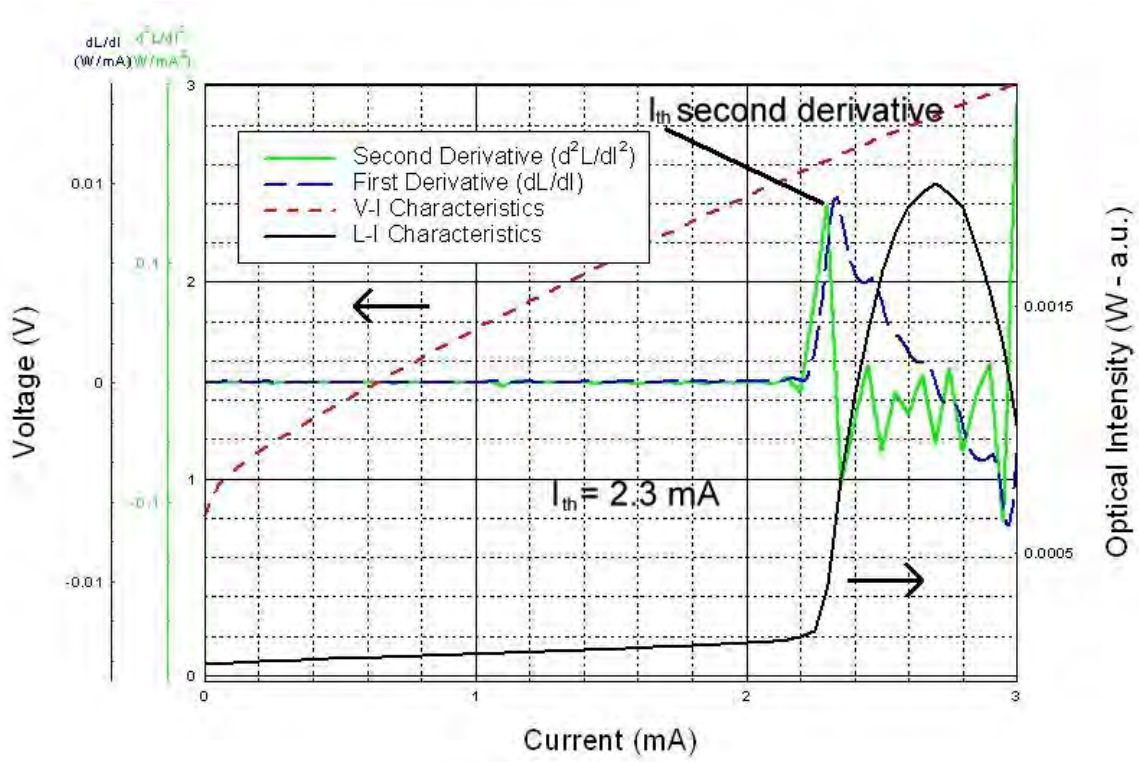
Figure 2.22: LIV curve of a QD VCSEL used to determine threshold current and slope efficiency
