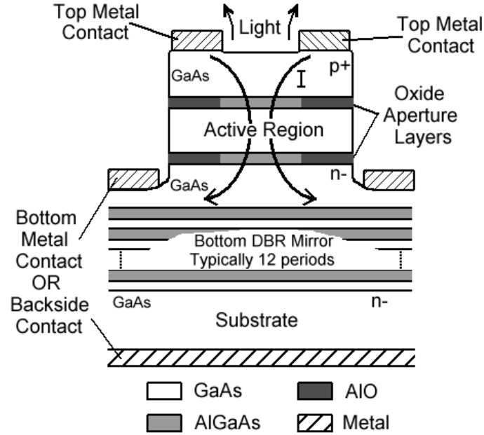
Figure 2.1: Structure of a typical RCLED
