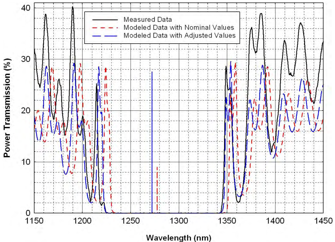
Figure 4.4: Measured power transmission of VCSEL DO177 compare to the modeled data
