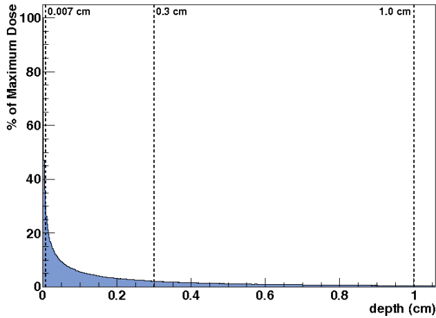
Fig. 19 Depth dose (0-100%) of an unfiltered 21.5 kVp spectra in tissue
