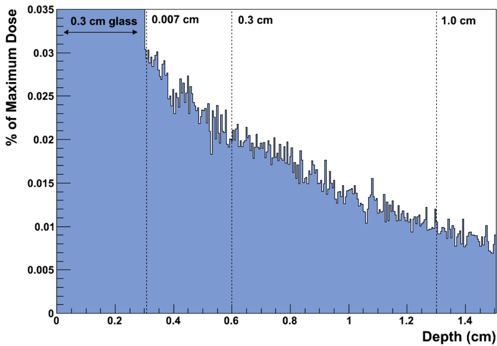
Fig. 21: Depth dose (0 – 0.03%) of a 0.3 cm glass window filtered 21.5 kVp spectra in tissue
