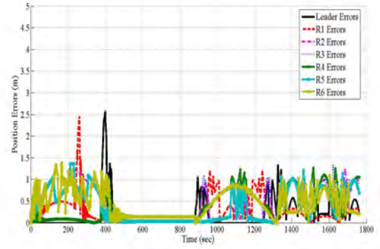
FIGURE 7: Sim (1) - Slave Position Errors
