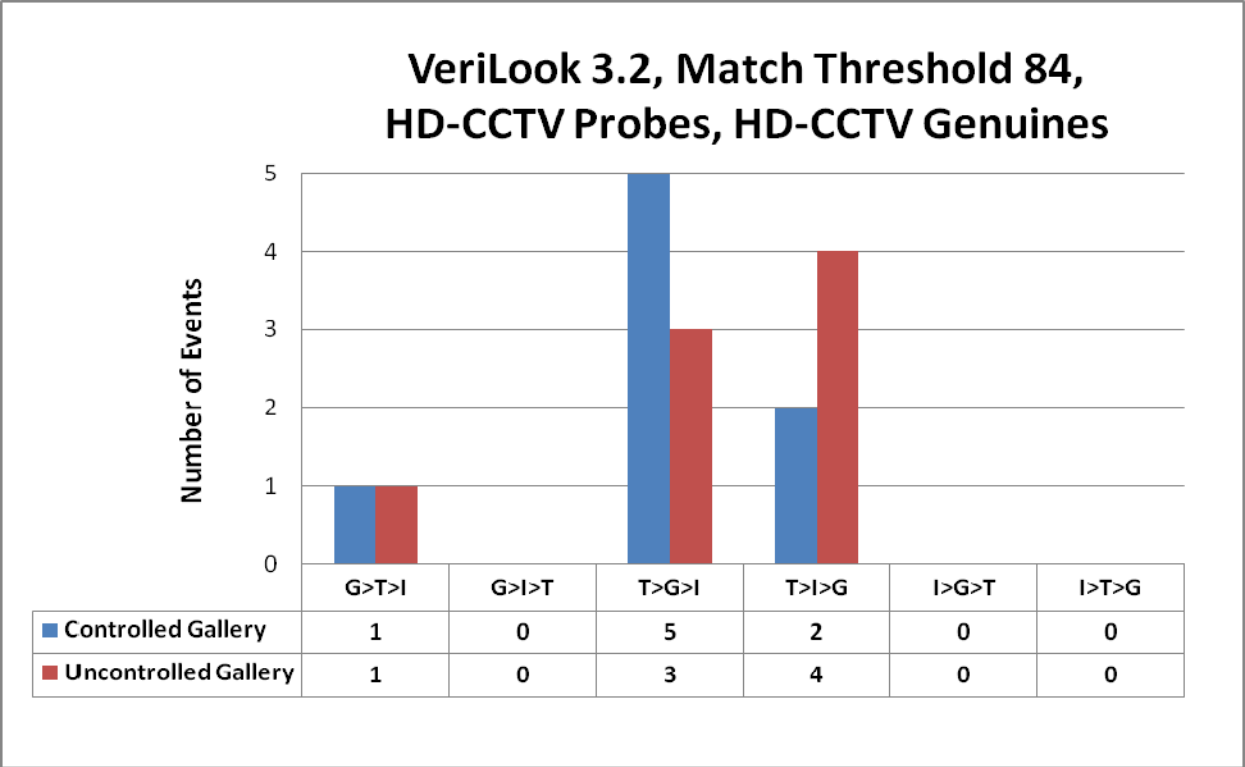
Figure 66: Default Threshold - Genuine and Impostor Results (VeriLook 3.2 / Genuine Passport Targets)
