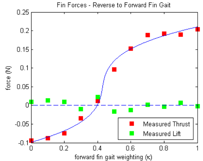
Fig. 6: A curve fit (see (5)) of experimental thrust data for a single isolated fin at zero free stream flow velocity as the fin gait is shifted from full reverse kinematics ( \kappa = 0.0 ) to full forward kinematics ( \kappa = 1.0 ).
