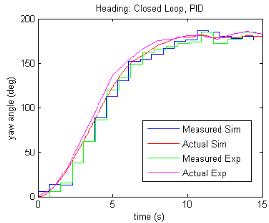
Fig. 16: Comparison of experimental and simulated closed-loop responses to a step change of 180^\circ in heading with PID control.
