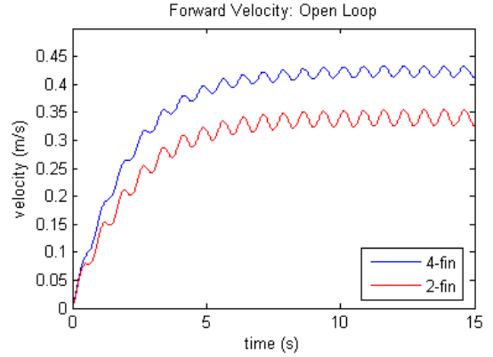
Fig. 13: Comparison of forward speeds of the two-fin and four-fin vehicles in simulation. The four-fin vehicle achieved 0.42 m/s whereas the two-fin vehicle achieved 0.34 m/s.
