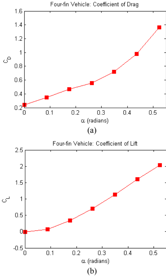
Fig. 3: (a) Vehicle drag and (b) vehicle lift coefficients computed for the four-fin vehicle at selected fixed angles of attack.
