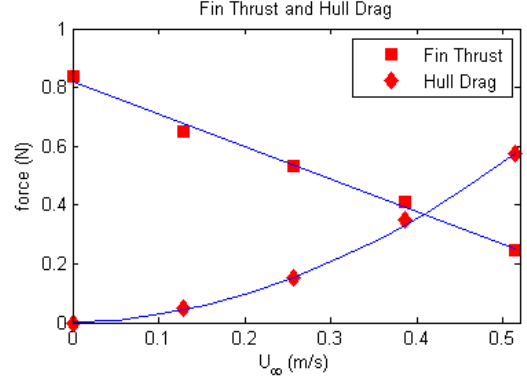
Fig. 12: CFD computed fin thrust and hull drag. The fitted data curves show the intersection where vehicle maximum forward velocity is reached.
