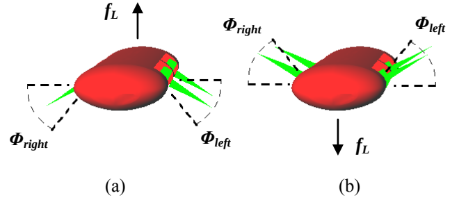
Fig. 5: Vehicle images showing all four fins with strokes (a) biased down to produce positive lift and (b) biased up to produce negative lift.
