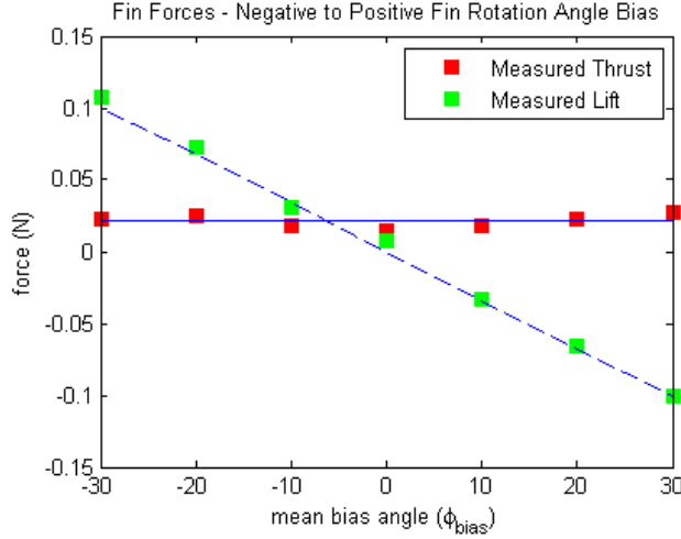
Fig. 7: A curve fit (see (6)) of experimental lift data for a single isolated fin at zero free stream flow velocity as the fin rotation angle bias is shifted from \Phi_{bias} = -30^\circ to \Phi_{bias} = 30^\circ . Fin gait weighting is set at \kappa = 0.4 for constant near zero thrust.
