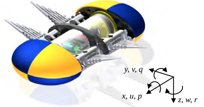
Fig. 2: Four-fin vehicle design with outer shell removed.
