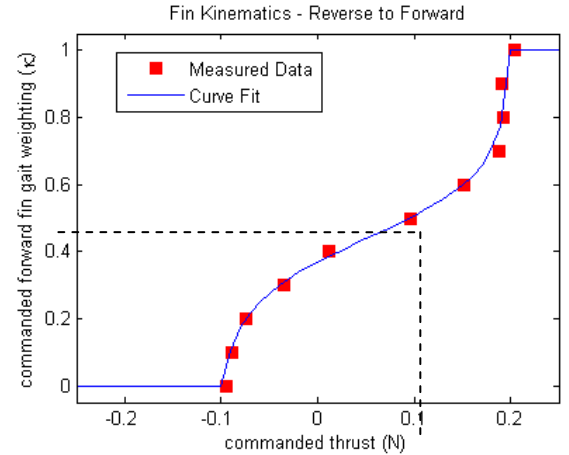
Fig. 11: A curve fit of experimental thrust data for a single isolated fin showing the necessary fin gait weighting as commanded thrust changes for each fin at zero free stream flow velocity.
