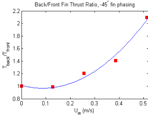
Fig. 9: CFD computed data showing the improvement in back fin thrust over front fin thrust at a -45^\circ back fin phase lag.
