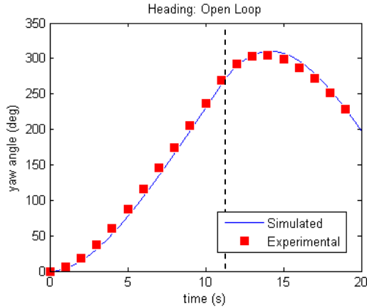
Fig. 14: Comparison of experimental and simulated open-loop heading angle responses.
