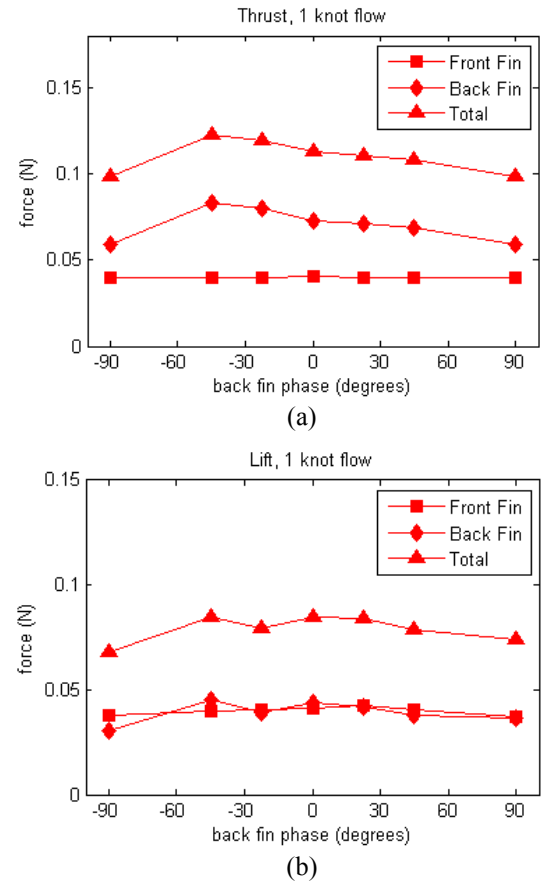
Fig. 10: (a) Thrust and (b) lift generated by front fin and back fin. At one knot flow, the vortices off the front fin give a boost to the thrust of the back fin for our particular configuration.
