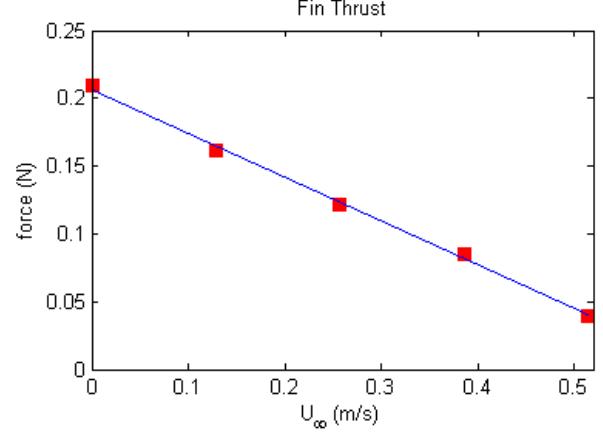
Fig. 8: CFD computed data showing thrust for a single isolated fin as a function of incoming flow velocity.
