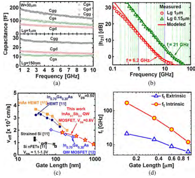
Fig. 4. (a) C_{gs} , C_{gd} , and C_{gg} as a function of frequency for devices with L_G = 150 nm and 1\ \mu\text{m} . High values of parasitic C_{gd} in these devices (due to incomplete isolation etch) limit RF performance, which could not be deembedded during the open calibration process. (b) Measured and modeled |h_{21}| as a function of frequency. (c) Extracted intrinsic v_{\text{eff}} versus gate length showing v_{\text{eff}} = 1.8 \times 10^7 cm/s for 150 nm L_G device, which is one of the highest effective velocities reported for III–V devices. (d) Intrinsic and extrinsic f_t versus gate length.
