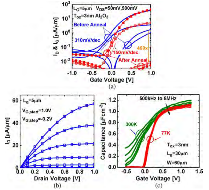
Fig. 2. (a) Transfer characteristics of the L_G = 5\ \mu\text{m} device. (b) Output characteristics of the L_G = 5\ \mu\text{m} device, showing very good saturation without any effect of impact ionization. (c) Split C-V characteristics at 77 K and 300 K.
