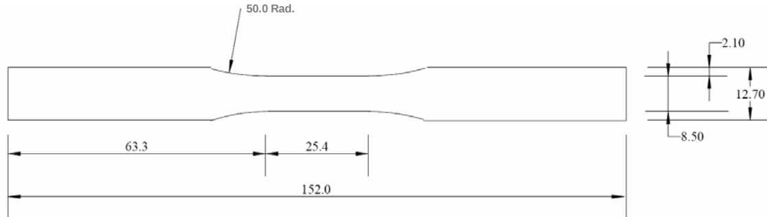
Fig 3: Specimen design (all dimensions in mm)
