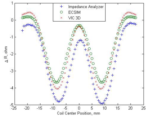
Figure 3b. Resistance for 7075 T6
