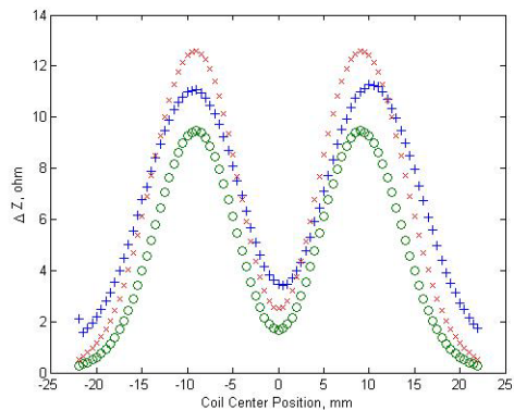
Figure 3f. Impedance for 7075 T6
