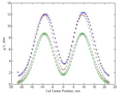
Figure 3d. Reactance for 7075 T6
