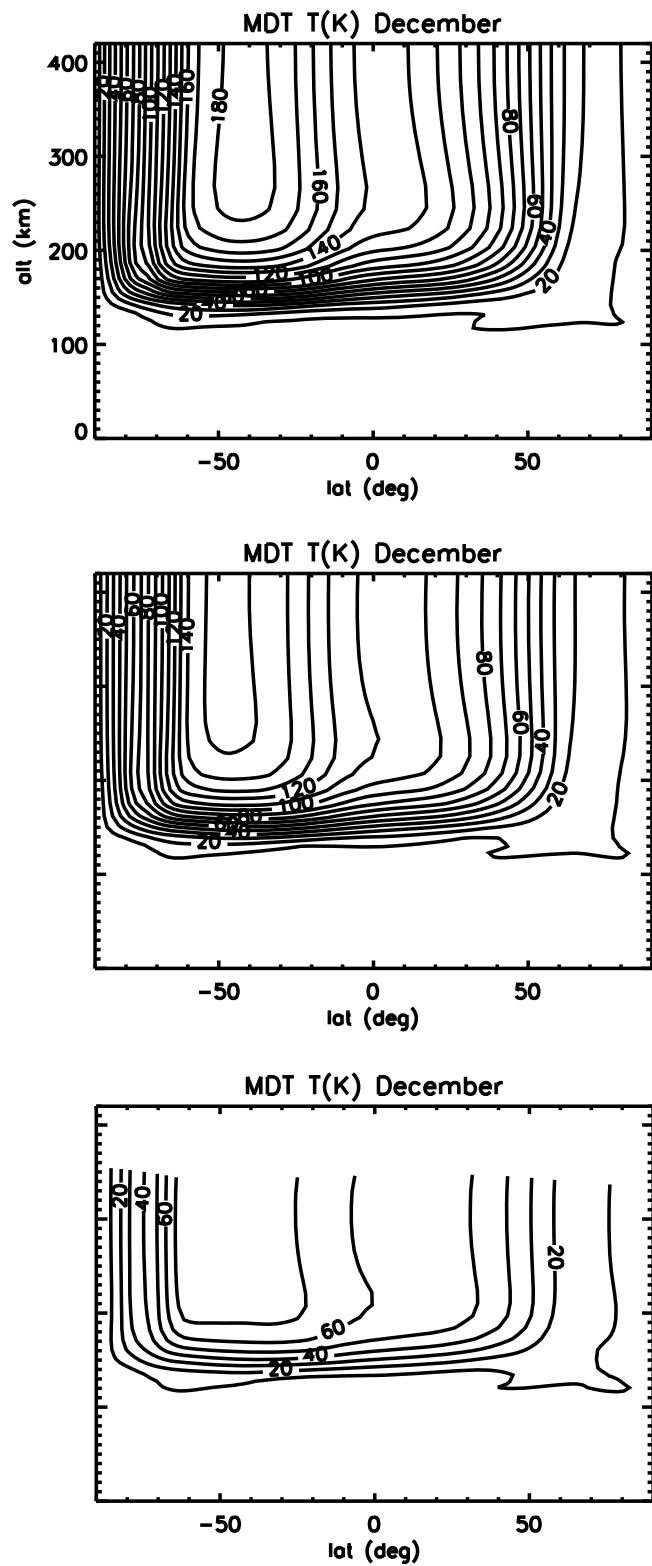
Figure 13. Migrating diurnal tide of temperature for December under (top) solar maximum, (middle) solar medium, and (bottom) solar minimum conditions. Contour intervals: 10 K.
