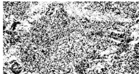
Figure 3. Crystal direction map for sample GKT where black grains have [0001] between 25° and 55° from the loading direction (vertical).
