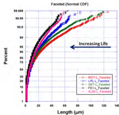
Figure 4. Cumulative distribution function showing time spent in facet forming orientations for six different conditions
