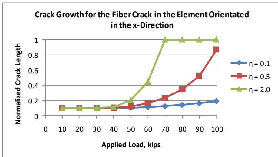
Figure 4. Normalized crack growth for the three values of \eta
