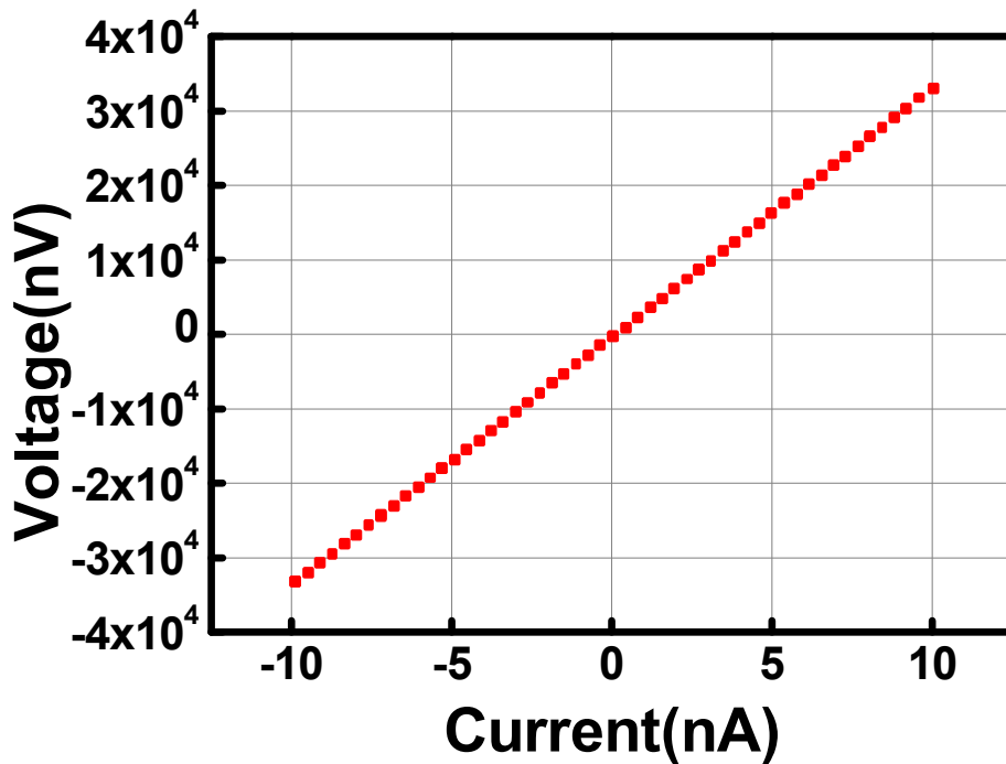
Fig. 5 Electrical resistivity of the individual nanowire at room temperature
