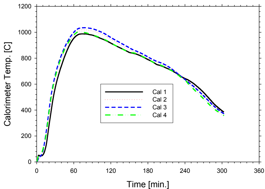
Figure 12. Test 6 calorimeter temperatures.
