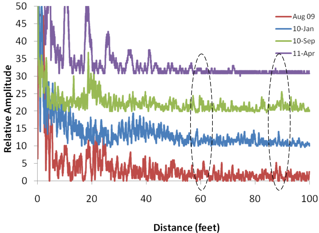
Figure 12. Monitoring changes in data sets obtained at the baseline and successive months by underground sensor #22532. An offset of ten units along the vertical axis has been added to each successive trace before plotting.
