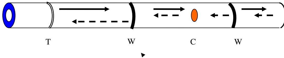
Figure 1. Sketch of ultrasonic guided wave propagation in a pipeline.
