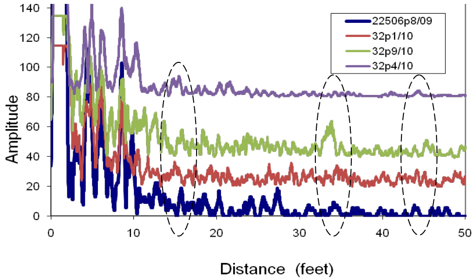
Figure 13. Monitoring signal changes in data sets obtained by above-ground sensor #22506. An offset of twenty units along the vertical axis has been added to each successive trace before plotting.
