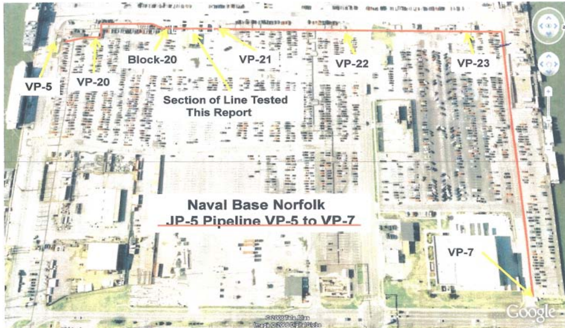
Figure 2. JP-5 pipeline layout (shown in red) from VP5 to VP7 at Norfolk Naval Station.
