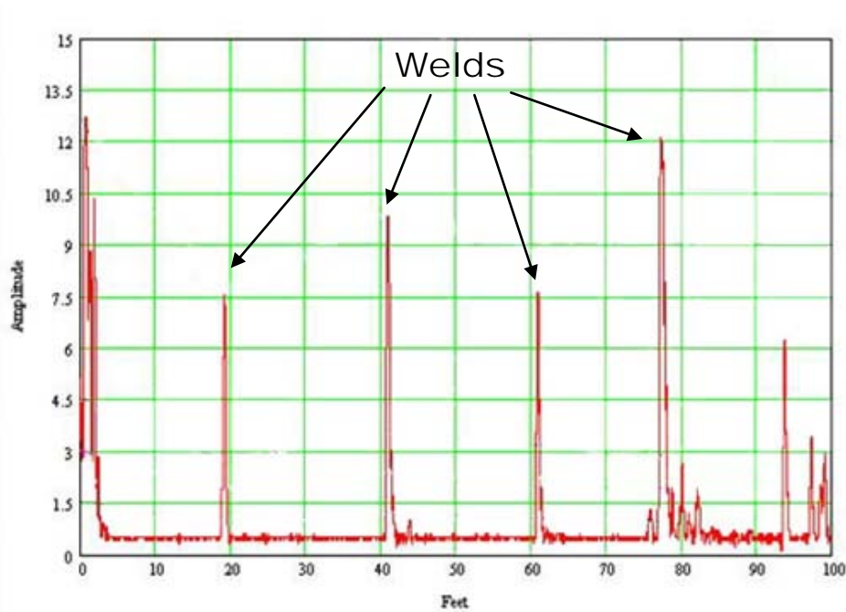
Figure 8. Example of plotted ultrasonic guided wave baseline data for the above-ground coating system pipeline at NSWCCD before corrosion was initiated. The plot shows peaks originating from welds, approximately 20 feet apart, as sensed by a transducer mounted in location 2.
