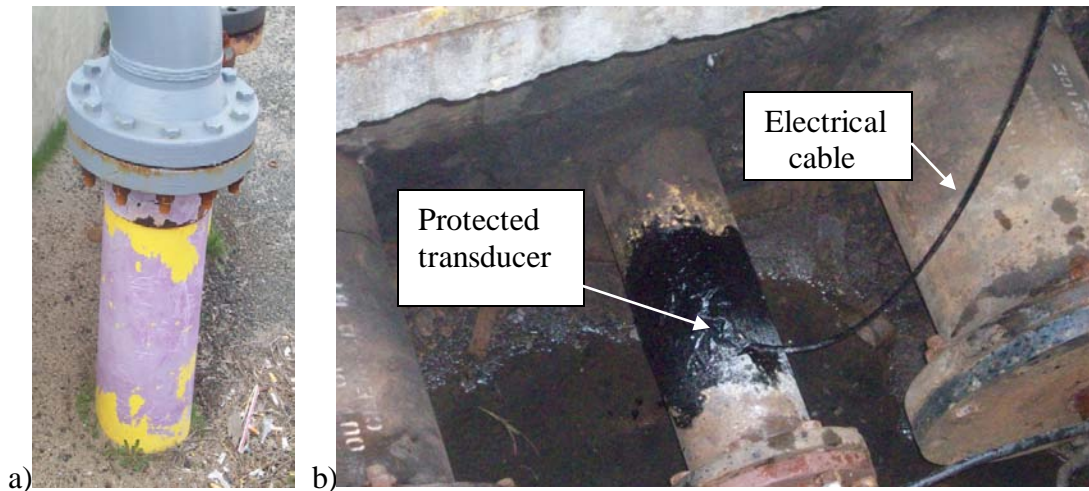
Figure 6. Surface conditions of tested pipe.
