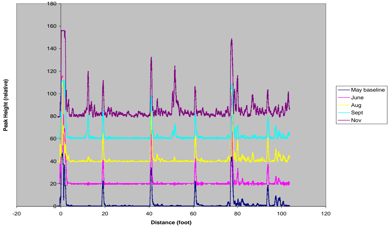
Figure 9. Systematic increases in defect detection over time as compared to the baseline. Systematic increases in peak heights for growing Defects 1 and 2 sensed by transducer at location 2. Defect 1 was located at approximately 50 feet and Defect 2 was located at approximately 12 feet. The other large peaks, approximately 20 feet apart, are from the welds in the pipeline. The baseline signal (May 2008) is blue, the June signal is pink, the August signal is yellow, the September signal is light blue, and the November signal is purple. An offset of twenty units along the vertical axis has been added to each successive trace before plotting.
