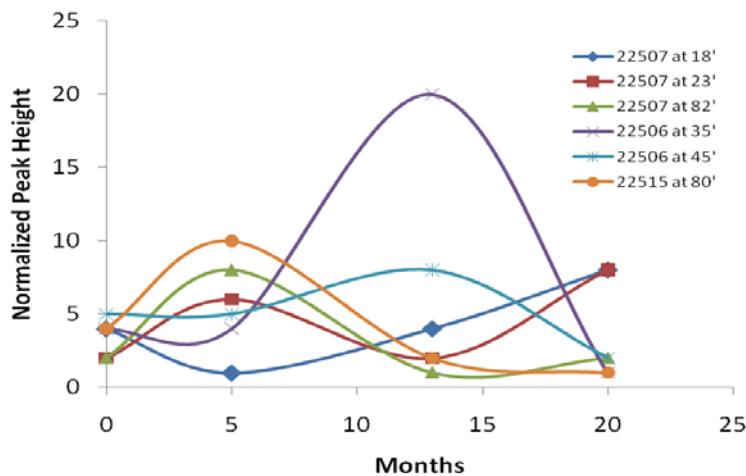
Figure 14. Changes in normalized peak height at suspected defect locations detected by three above-ground transducers. Typical signal noise was 2 vertical units.
