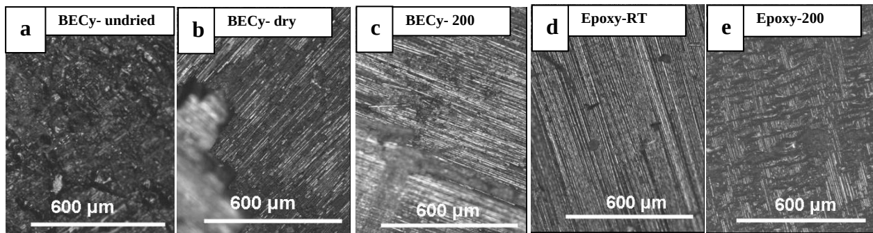
Figure 28. Microscopic images of fracture surface of BMI-cf lap shear specimens demonstrating the various modes of failure under different testing conditions for a) BECy-undried and b) BECy-dry c) BECy-200 d) Epoxy-RT e) Epoxy-200.
