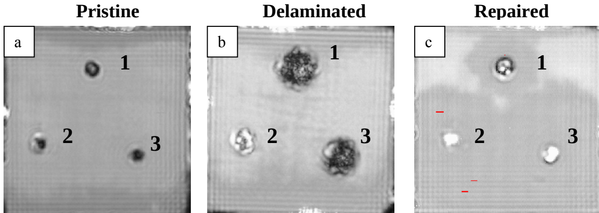
Figure 43. C-scan images of 10 in x 10 in BMI-cf PMC panel, a) Pristine, b) Delaminated, c) Repaired
