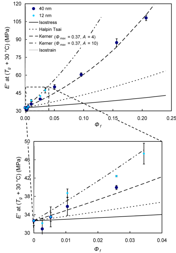
Figure 61. Rubbery storage modulus (@ T_g + 30\text{ }^{\circ}\text{C} ) vs. volume fraction.
