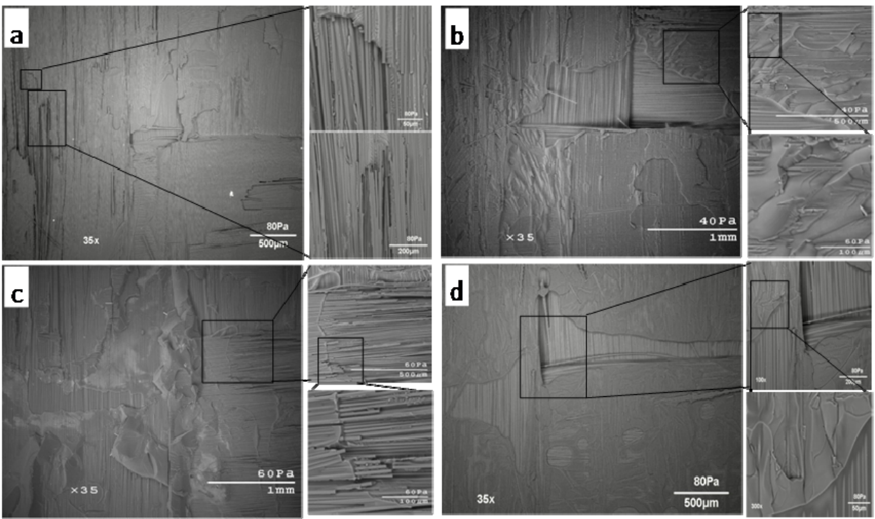
Figure 32. SEM images of DCB fracture surfaces a) Pristine sample, b) Wet repaired sample, c) Dry repaired sample d) Epoxy repaired sample at 200 °C
