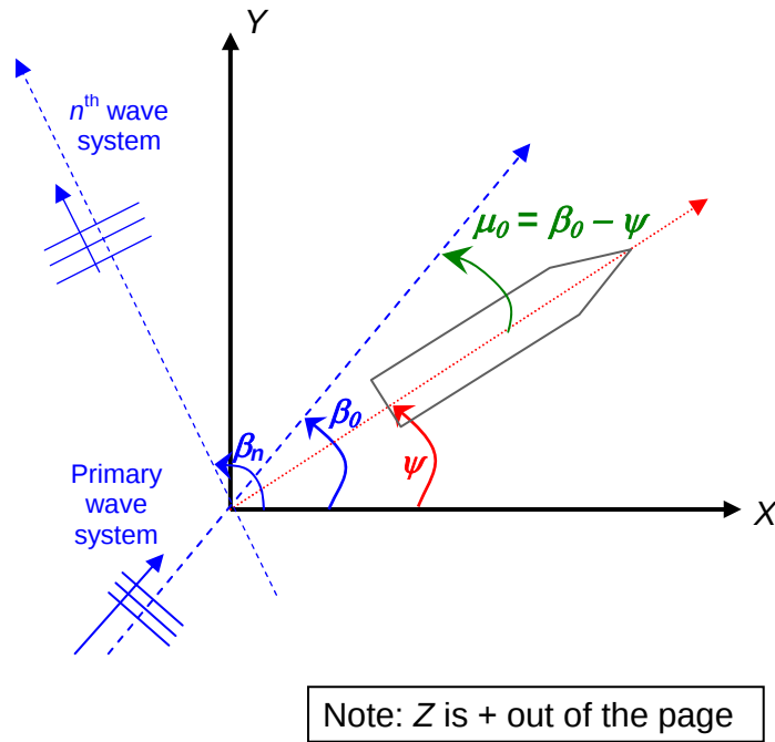
Figure 3-2 Definition of ship heading and wave heading angles
