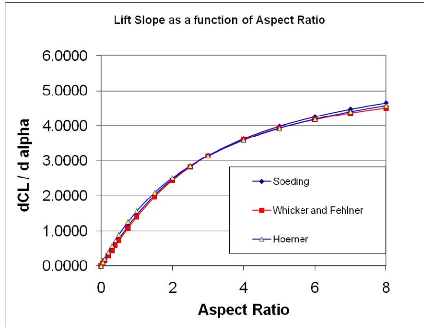
Figure 6-4 Comparison of formulae for lift coefficient slope.
