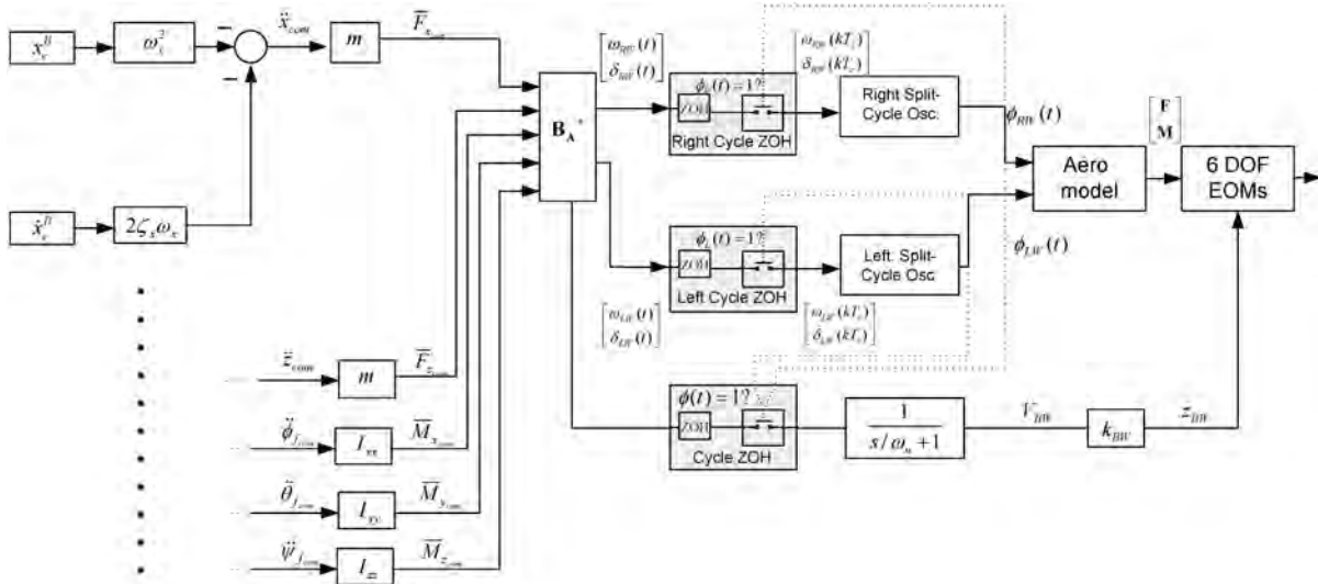
Fig. 6 Five-degree-of-freedom split-cycle controller.
