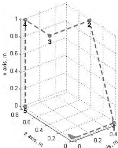
Fig. 7 Desired trajectory.
