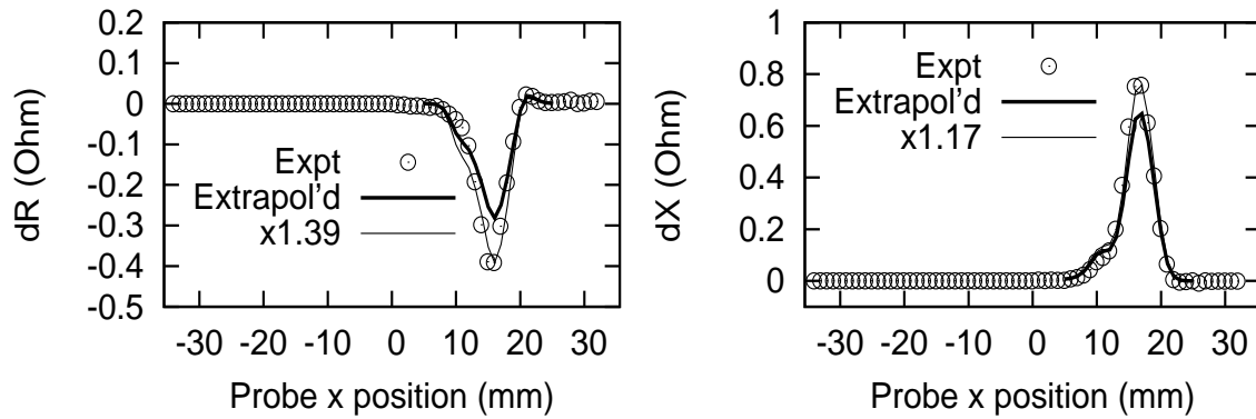
Notch at a Bolt Hole Benchmark Problem 1 Notch at a Bolt Hole Benchmark Problem 1
