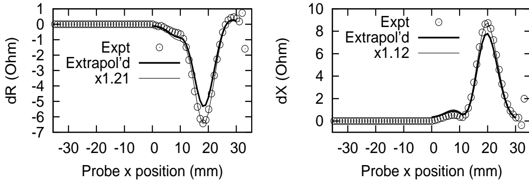
Notch at a Bolt Hole Benchmark Problem 2 Notch at a Bolt Hole Benchmark Problem 2
