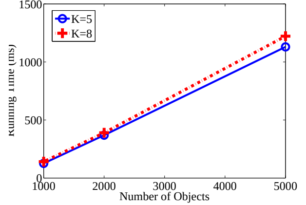
Figure 7.4: Running Time
