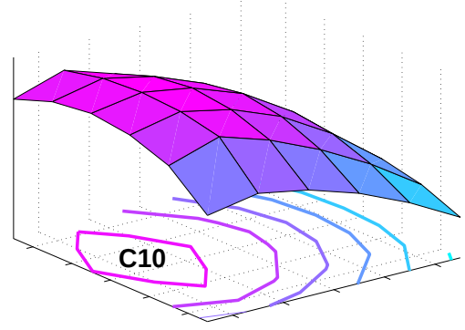
Figure 8.9: Updated Transitions
