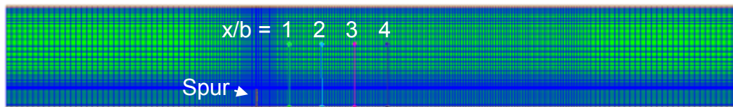
Figure 16. CMS-Flow computational grid for the spur-dike case. Colored lines represent the location of where calculated current velocities in the x-direction were extracted and compared to measurements (see Figure 17).
