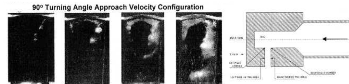
Figure 20: Sequence from Inception of Cavitation to Full Cavitation [18]
