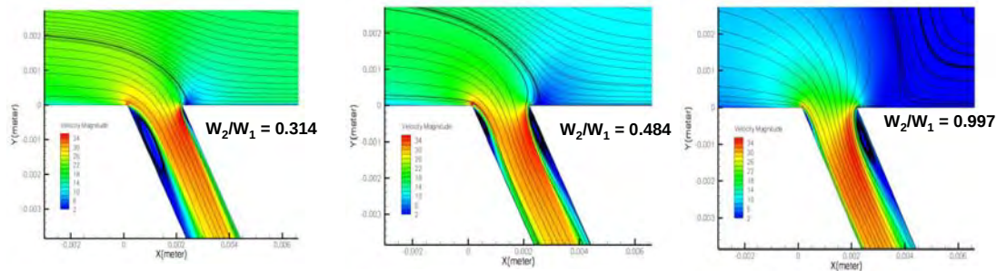
Figure 13: CFD Flow Characteristics for 60° Turning Angle 2D Orifice
