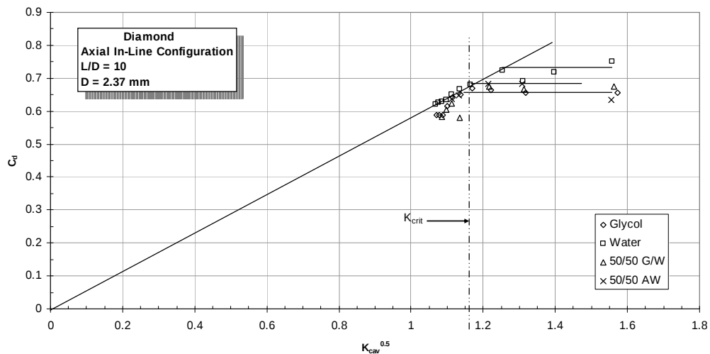
Figure 47: Cavitation Characteristics for Several Fluid Combinations [27]
