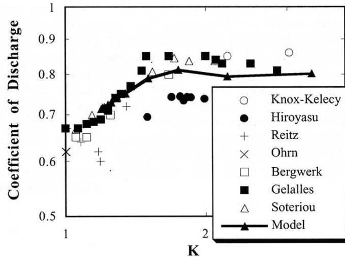
Figure 54: Experimental Coefficient of Discharge Comparison with Theory [41]
