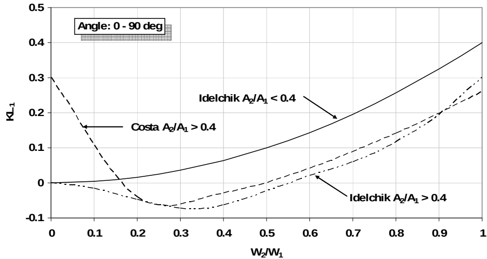
Figure 15: Impact of Flowrate Ratio on Manifold Loss Coefficient in Manifold/Orifice Deceleration – Idelchik [1] & Costa [11]
