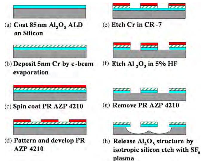
Fig. 3. Fabrication process of ALD-based resonator.
