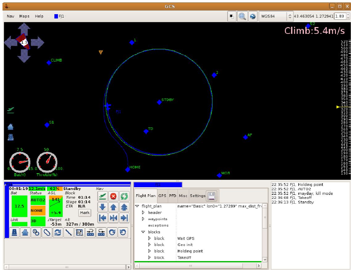
Figure 47 - The Paparazzi Ground Control Station (GCS)
