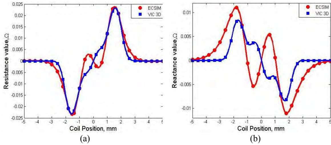
FIGURE 3. Results for generic Air Cored Split D Differential, (a) \Delta R , (b) \Delta X
