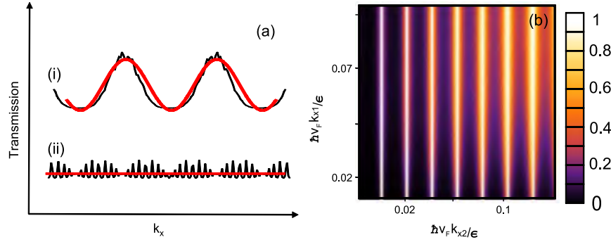
Figure 4. Effect of disorder on the transmission probability using the Lorentzian distribution model. In panel (a) we plot in (i) the transmission probability as a function of k_{x1} for dressed electrons (black curve) compared to infinite graphene (red curve) for head-on collision. The plot in (ii) shows a two-peak model distribution under the influence of disorder. In panel (b) we show the transmission probability for electron dressed states with \Delta = V_0/3 in the presence of disorder.
