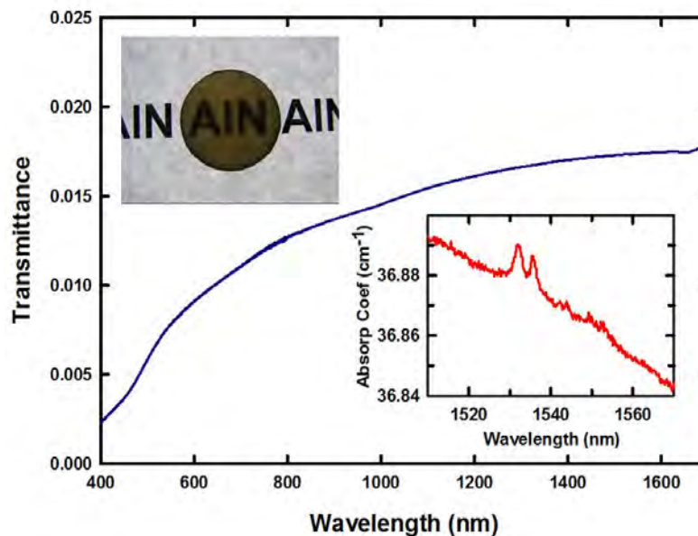
Fig. 1. Transmittance (as a fraction, not percent) of 1.15 mm thick sample of Er:AlN ceramic. Upper left inset: 1 mm thick sample, backlit. Lower right inset: Absorption coefficient in the region of \text{Er}^{3+} {}^4\text{I}_{13/2} absorption.
