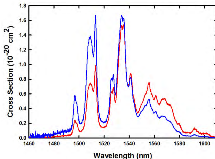
Fig. 10. Room temperature stimulated emission (red trace) and ground state absorption (blue trace) spectra of \text{Er}^{3+} in the presumed dominant site of \text{Er:AlN} .
