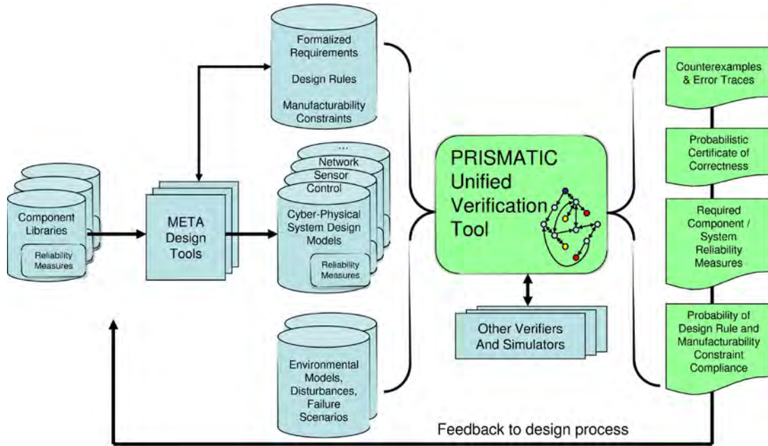
Figure 1: Cyber-physical System Design with PRISMATIC
