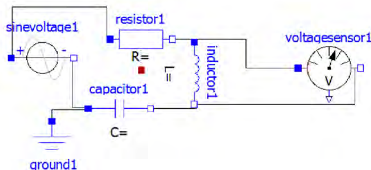
Figure 4: Example RLC Circuit, Modeled in OpenModelica's OMEdit
