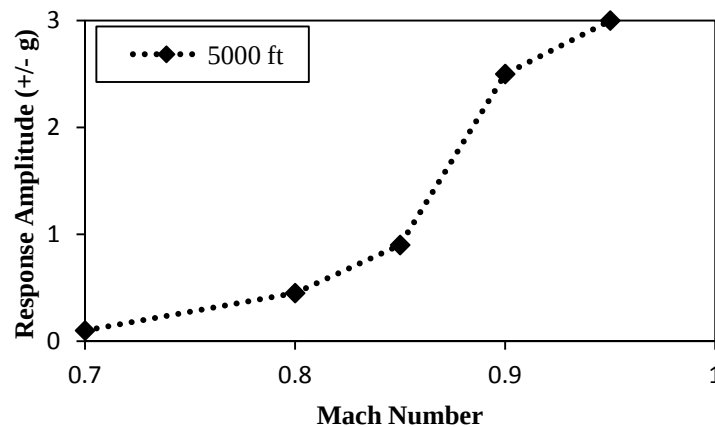
Figure 1. LCO Response Amplitude at 5000 Feet MSL Altitude.
