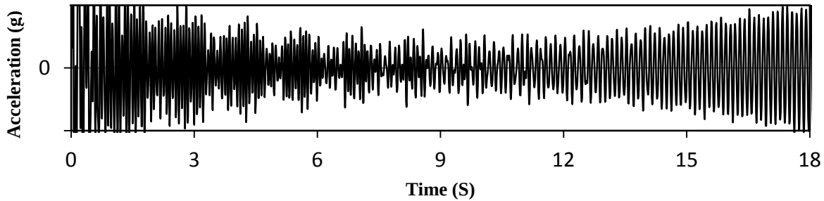
Figure 8. Mach Number 0.75 Structural Response Time History.
