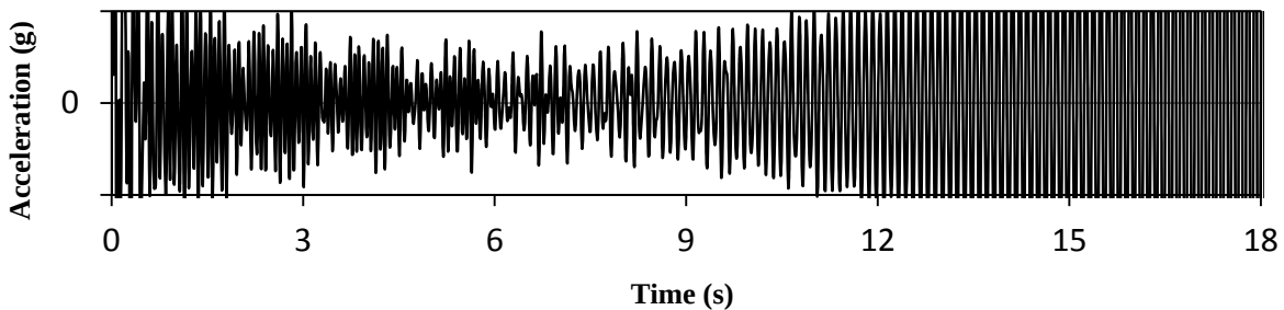
Figure 9. Mach Number 0.80 Structural Response Time History.
