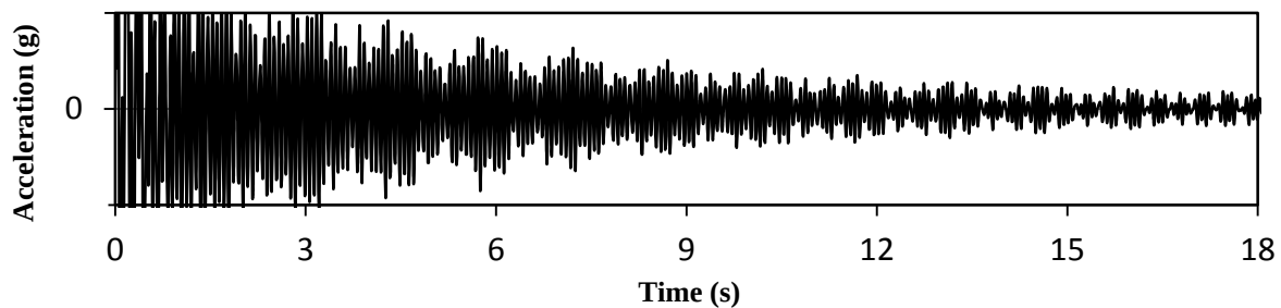
Figure 6. Mach Number 0.65 Structural Response Time History.
