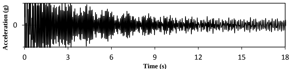
Figure 7. Mach Number 0.70 Structural Response Time History.
