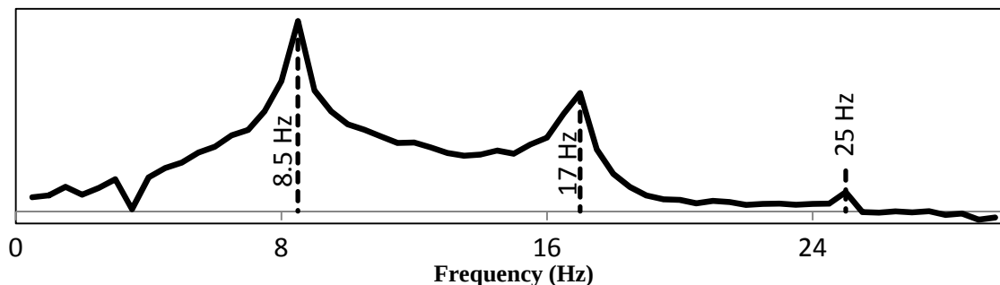
Figure 11. FFT of Pressure Data from Prescribed Structural Motion Simulation at a Point Behind Wing-Tip Launcher Rail.
