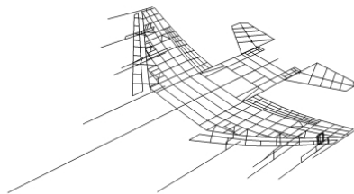
Figure 3. 1st Mode Shape.
