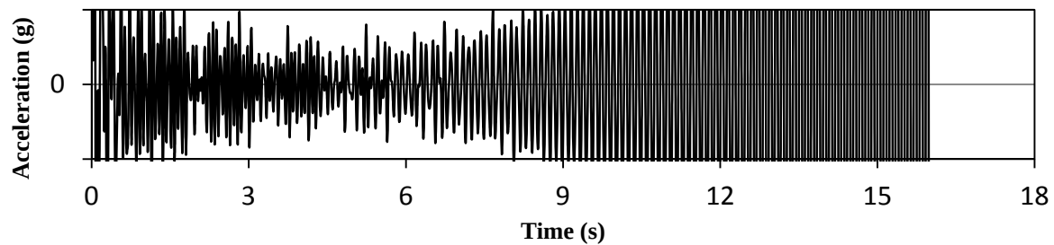
Figure 10. Mach Number 0.85 Structural Response Time History.
