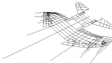
Figure 4. 2nd Mode Shape.
