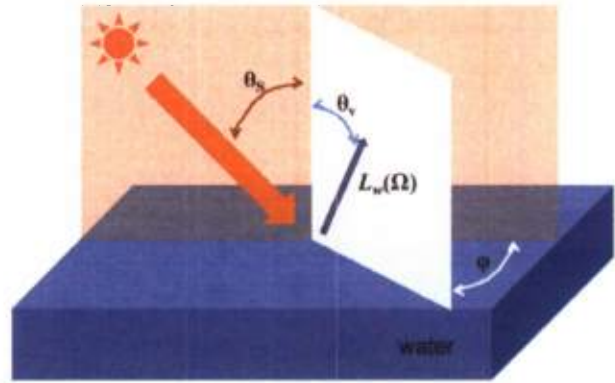
Fig. 1. (Color online) Angular coordinate used in this study and the IOP-centered system.
