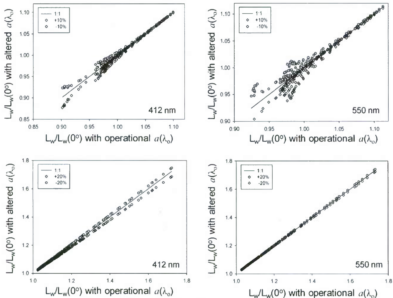
Fig. 9. Scatter plot of L_w(\lambda, \Omega)/L_w(\lambda, 0^\circ) for different values of a(\lambda_0) . The x axis represents the L_w(\lambda, \Omega)/L_w(\lambda, 0^\circ) ratio derived with a(550) in the current QAA scheme; the y-axis represents the L_w(\lambda, \Omega)/L_w(\lambda, 0^\circ) ratio derived after altering the estimated a(550) . Top panel, the blue water in the Mediterranean Sea, a(550) was altered by \pm 10\% ; bottom panel, the green water in the Monterey Bay, a(550) was altered by \pm 20\% .
