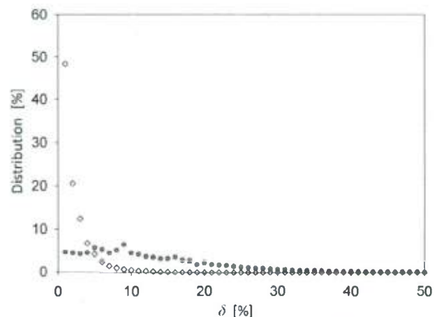
Fig. 4. Distribution of absolute percentage difference ( \delta ) of L_w . Simulated data were used, and focused on the angular domain that \theta_S = 60^\circ , \theta_v = 30^\circ – 70^\circ , and \varphi = 0^\circ – 180^\circ . Solid circle, no BRDF correction; open diamond, after IOP-based BRDF correction.
