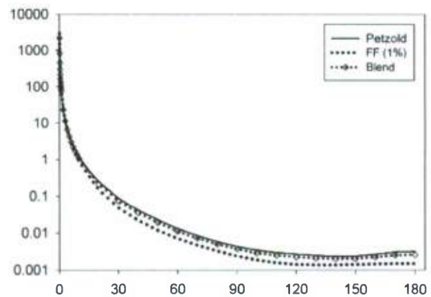
Fig. 2. Particle phase function shapes (Petzold average and 1% Fournier and Forand) used for the numerical simulation. The open diamond represents one weighted average of the particle assemblage.
