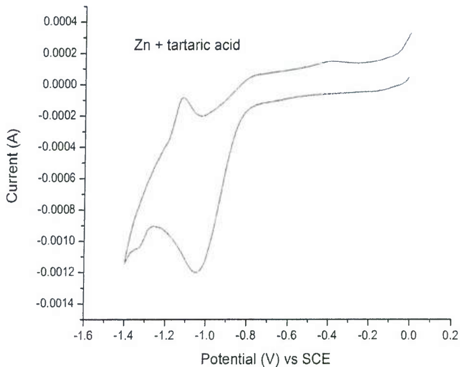
Figure 22. Cyclic voltammogram of 5 mM \text{ZnSO}_4 + 0.25 M tartaric acid.
