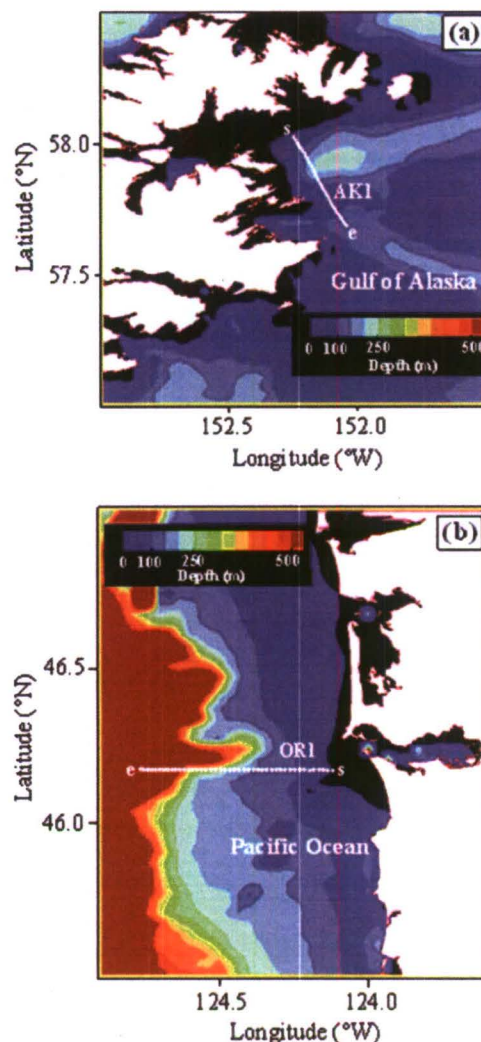
Fig. 1. (Color online) Geographic location of lidar surveys. (a) Eastern shelf of Afgonak/Kodiak Islands, (b) Western shelf off the Oregon/Washington coast. AK1 and OR1 are the airborne transects matching 1.1 km satellite ocean color data (white dots), land (white), and bathymetry with 1/30 deg resolution (color contours), missing data (black areas). Flight direction is indicated based on initial (s) and final (e) sampling locations.
