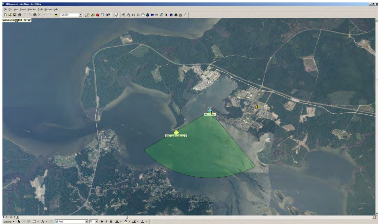
Figure 5. COT display showing the Compact Radar detecting a target entering the AO. Note that the entire choke point is monitored by the unit.
