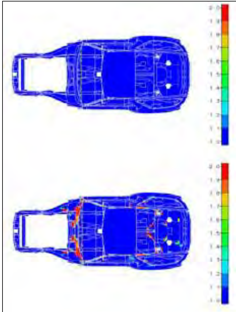
Figure 2. Topometry optimization (6).
