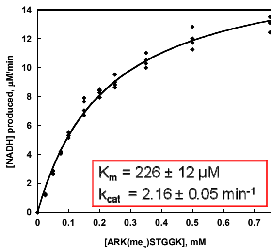
Figure 2. Michaelis-Menten plot of JMJD2E obtained by the fluorescence coupled assay. Reaction conditions: 20 mM Tris pH 7.4, 500 \mu M \alpha -KG, 500 \mu M ascorbate, 50 \mu M Fe(II)SO 4 •6H 2 O, 50 mM NaCl, 0.04 units FDH, 2 mM NAD + , 8 \mu M JMJD2A/C/E; varying ARK(me 3 )STGGK peptide concentrations.
