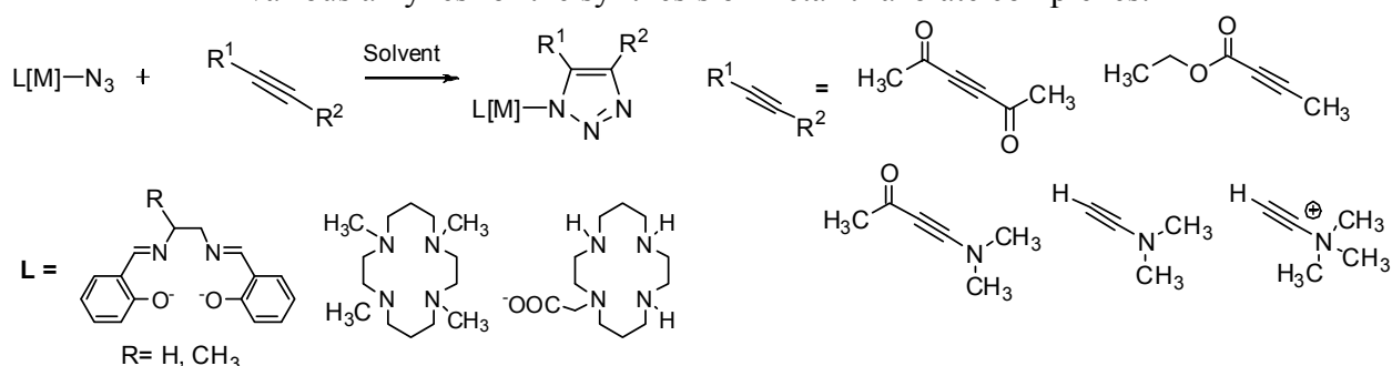
Scheme 2. The scope of the studied cycloaddition reaction between metal-azide complexes and various alkynes for the synthesis of metal-triazolate complexes.
