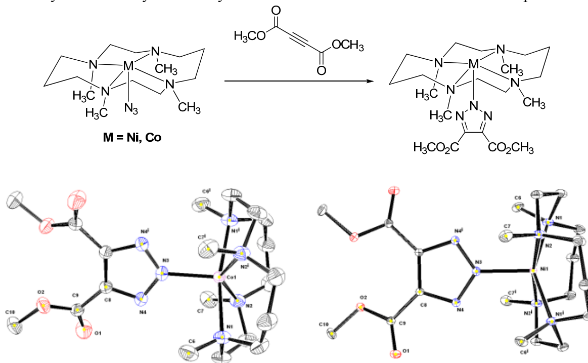
Scheme 3. Successful cycloaddition reaction between metal-azide complexes and dimethyl acetylenedicarboxylate and crystal structure of the Co- and Ni-triazolate complexes.
