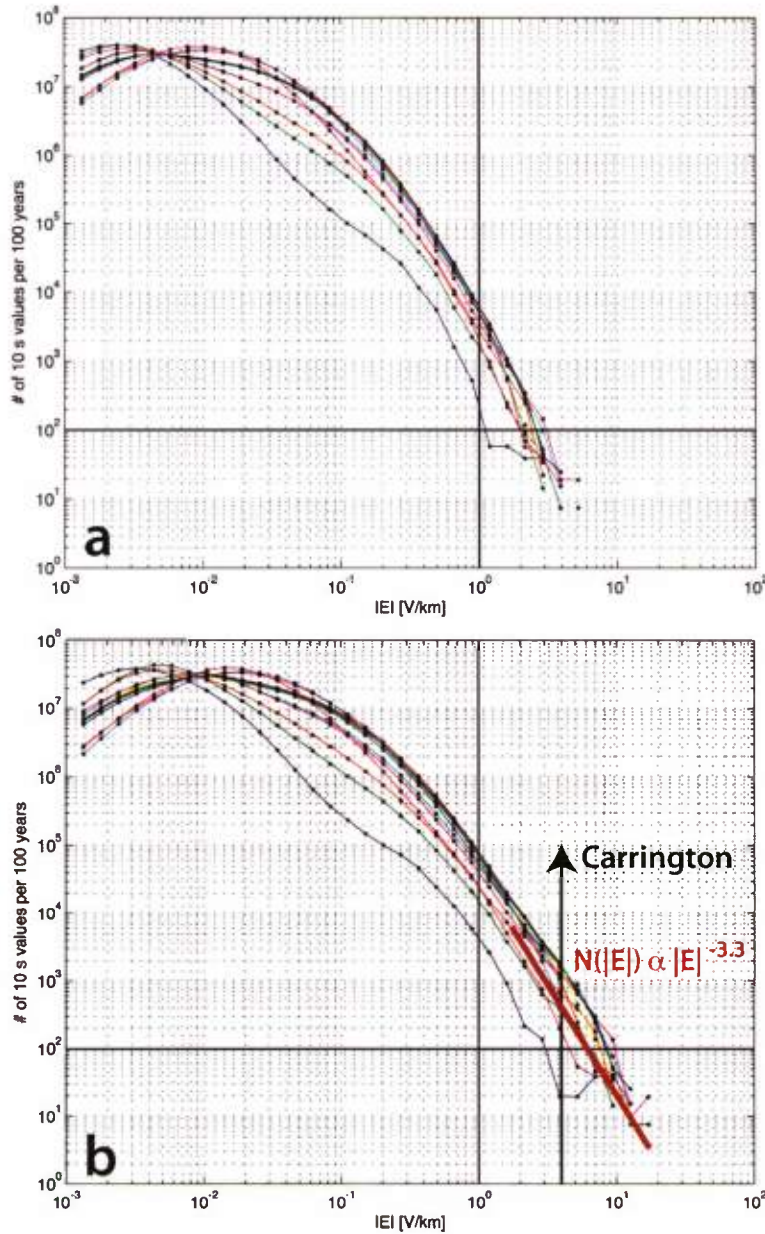
Figure 9: Number of 10 s geoelectric field magnitudes, |E| , produced by CME per 100 years, adapted from [41]. The estimates were made using simultaneous observations of GIC and geomagnetic fields in Finland with low and high-resistivity ground models characteristic of British Columbia (a) and Quebec (b). Each curve represents data from a different site. The arrow at 4 V/km marks the estimated magnitude of the Carrington Event, and the red line approximates power-law slopes at high magnitudes.
