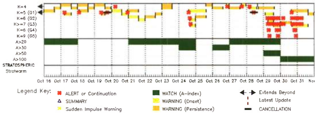
Figure 28: Summary of geomagnetic alerts, watches, and warnings issued by NOAA's Space Weather Prediction Center during the second half of October 2003. Elevated activity culminated in the Halloween Storms at the end of the month.
