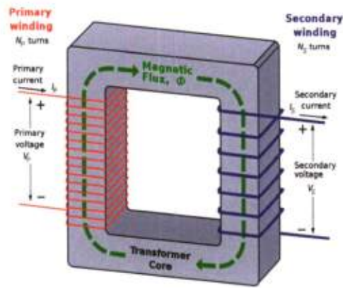
Figure 15: An ideal step-down transformer. After Wikipedia, Transformers, http://en.wikipedia.org/wiki/Transformer .
