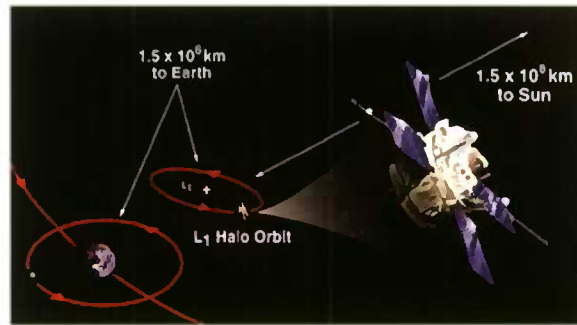
Figure 33: Advanced Composition Explorer (ACE) launched in 1997 into a halo orbit about L1.
