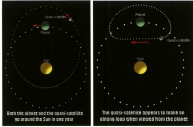
Figure 34: Schematic of a quasi-satellite orbit around the sun and the earth. The left panel shows a snapshot of the orbits from above the plane of earth's orbit. The satellite's orbit is much more elliptical than earth's. The right panel shows the apparent satellite orbit appearing to revolve around earth as seen from the planet.
