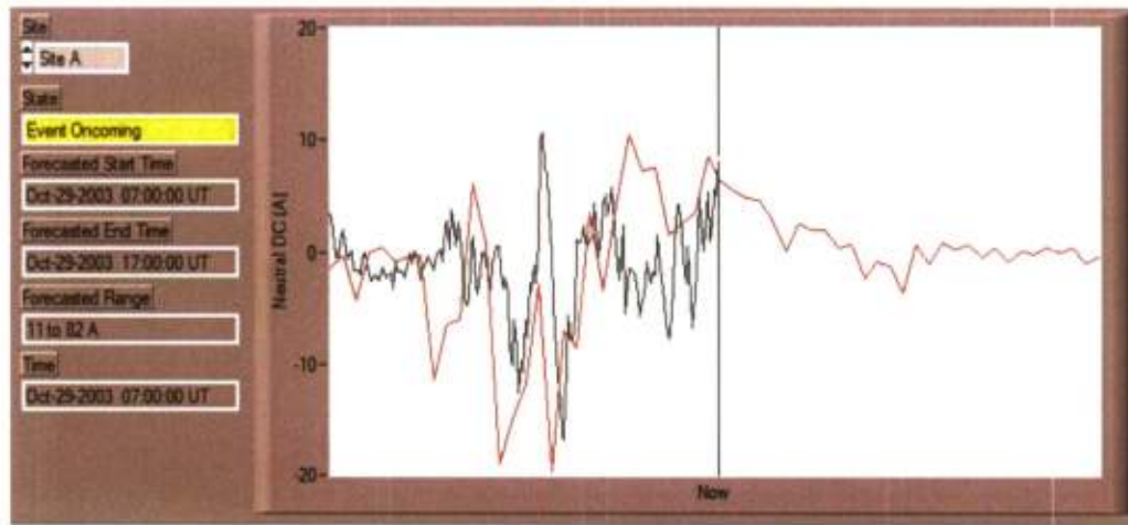
Figure 29: EPRI/NASA space weather warning during the 2003 Halloween solar storms. The Level One warning, in text boxes on the left, estimates a magnitude range of the GIC and its start and end times. The Level Two warning, on the right, compares predicted (red) and observed (black) GIC at a particular grid location.
