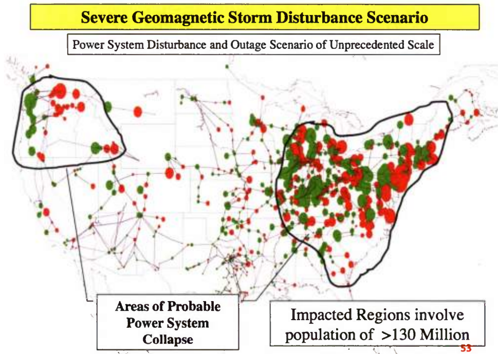
Figure 22: Summary of worst-case scenario disruption of the U.S. electric grid by a severe geomagnetic storm centered at 50°N (J. Kappenman presentation to JASON, 16 June 2011). Red and green circles indicate magnitudes of GIC into and out of transformers from the ground.
