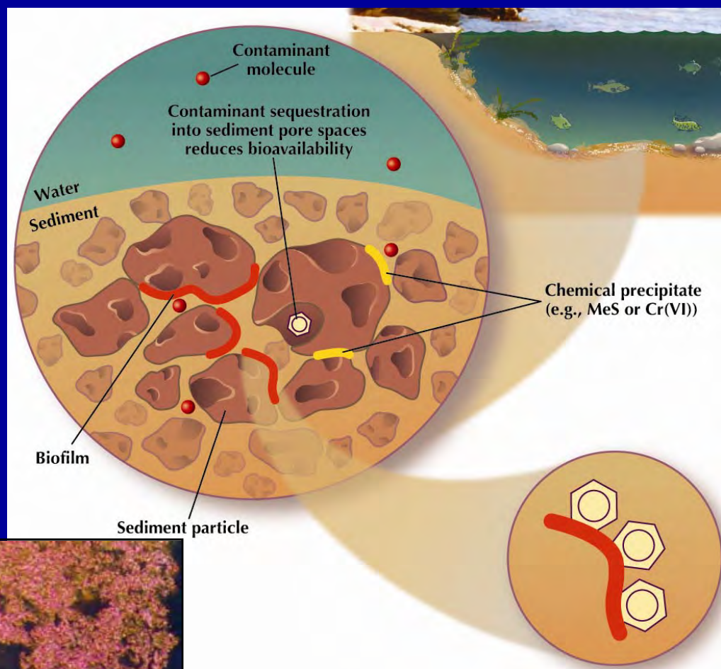
soot carbon
