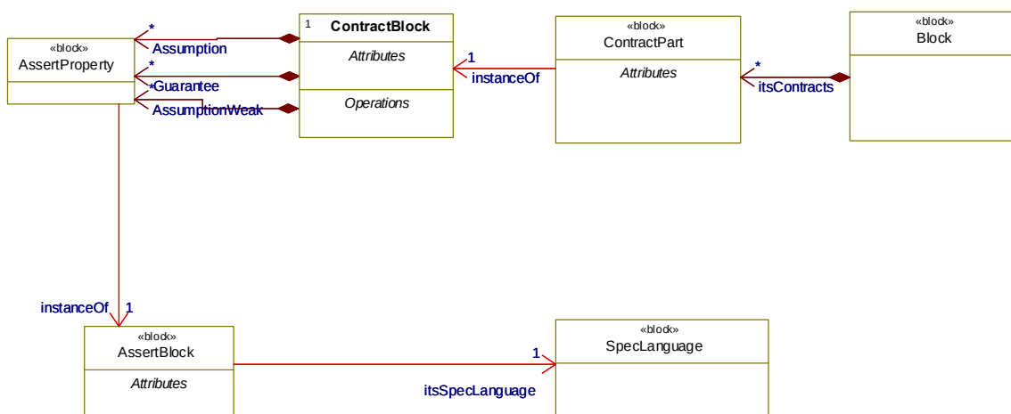
Figure 18 - Contracts Meta-model
