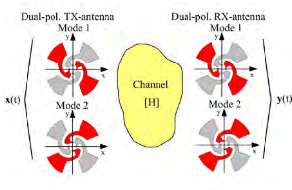
Figure 25: 2 \times 2 dual-mode MIMO [9].
