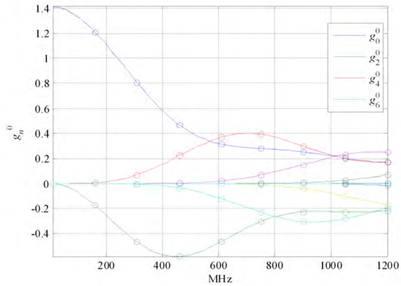
Figure 22: Uniform current (Legendre coefficients and 9-point splines).
